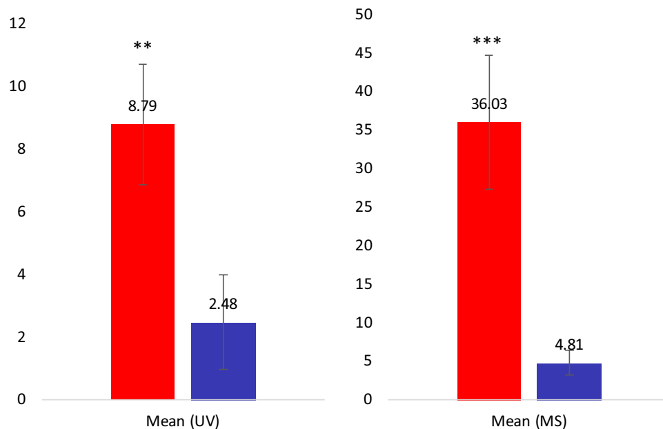
Figure 3. Mean HHQ/HQNOC9:1 ratio \pm SEM detected in chronic strains (PC + PCM, n=20 ; in red) and in first colonisation strains (PP + PF, n=19 ; in blue), using both UV (left) and HRMS (right) data. Significant differences were found by using Kruskal–Wallis tests ( \chi^2=8.7066 , df=1 , p -value = 0.003171 for UV, and \chi^2=18.723 , df=1 , p -value = 1.511 \times 10^{-5} for HRMS).
