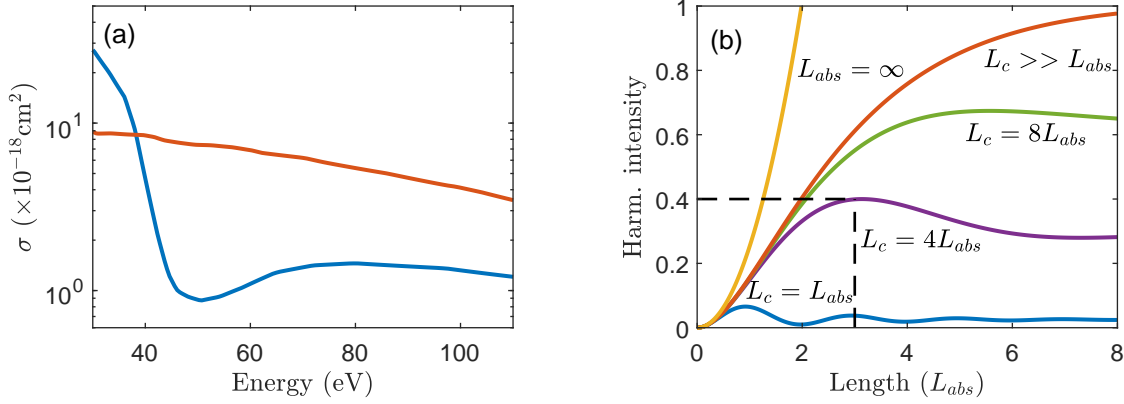
Figure 5. Influence of absorption (a) Absorption cross section as a function of photon energy in Ar (blue) and Ne (red). Data from 62 . (b) Harmonic intensity as a function of medium length in units of L_{\text{abs}} for different coherence lengths [ L_c = L_{\text{abs}}, 4L_{\text{abs}}, 8L_{\text{abs}}, and L_c \gg L_{\text{abs}} (blue, violet, green, red)]. The yellow line indicates the harmonic intensity calculated without absorption. The dashed black lines indicate at what medium length the maximum harmonic intensity is obtained for the case L_c = 4L_{\text{abs}} , which is related to the fit parameter \zeta = 3 introduced in Eq. (32). [adapted from E. Constant (1999)].
