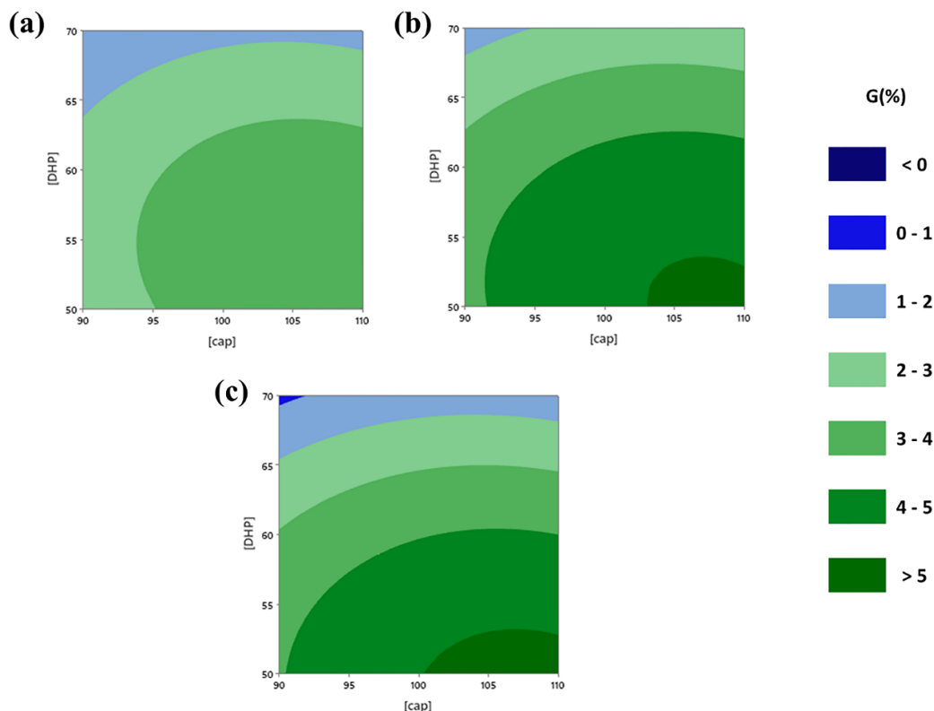
Fig. 5. Contour plots showing the combined effect of microcapsules and DHP CATs on the mass gain ( G ) using different CA crosslinking agent concentrations: (A) 80 g · L -1 , (B) 100 g · L -1 and (C) 120 g · L -1 . CAT, catalyst concentration; DHP, disodium hydrogen phosphate
