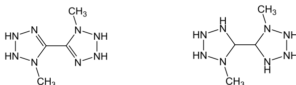
Figure 5. Structures of 1,1'-dimethylbistetrazoline ( M = 170\text{ g}\cdot\text{mol}^{-1} ) and 1,1'-dimethylbistetrazolidine ( M = 172\text{ g}\cdot\text{mol}^{-1} ), respectively.
