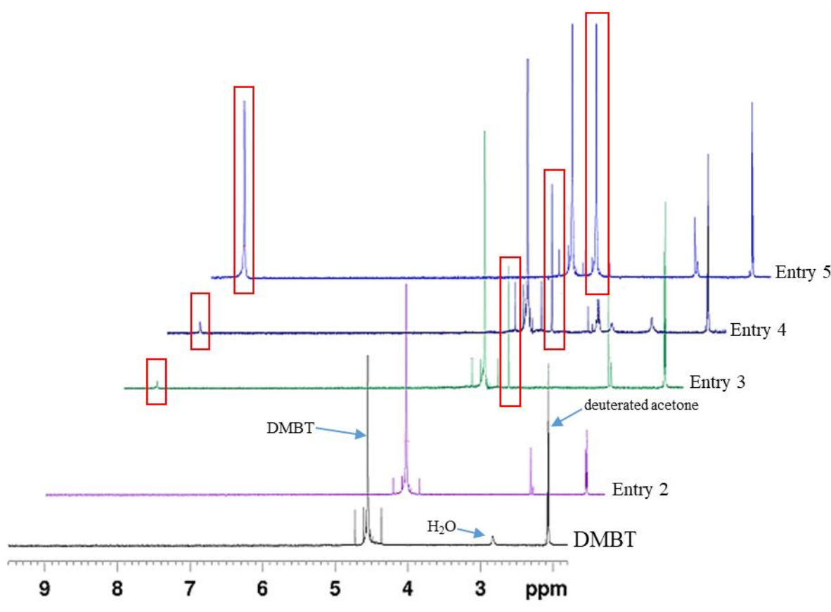
Figure 4. Superposition of ^1H NMR spectra (400 MHz), in deuterated acetone, for DMBT and reaction crude.
