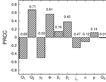
Fig. 4 Sensitivity analysis of \mathcal{R}_0 . The parameters Q_1, Q_2, Q_3 are respectively \bar{A}_1/\gamma_A, \Omega/\gamma_X and a dummy parameter.
