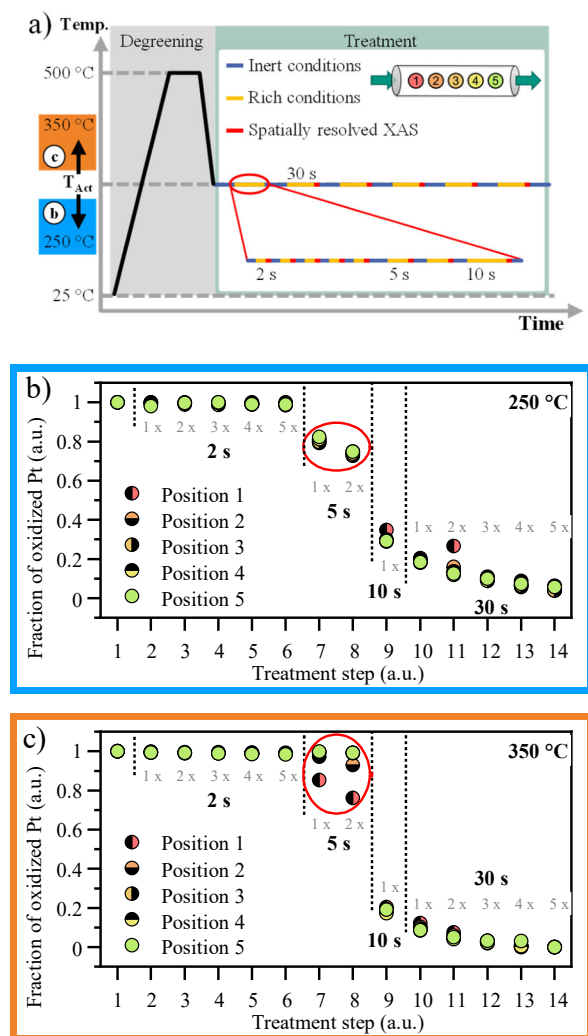
Figure 7. (a) Schematic sequence for the stepwise reduction of the Pt/CeO 2 /Al 2 O 3 catalyst; oxidation state of Pt after treatment steps with reductive pulses (2% CO in He) in an inert atmosphere (He) ranging from 2 s to 30 s at (b) 250 °C and (c) 350 °C. The fraction of oxidized species is presented spatially resolved at 5 positions along the catalyst bed ranging from its inlet (red) to the outlet (green) and estimated by LCA of the spatially resolved XANES. The spectra were normalized to the lean treated sample and after complete reduction at the respective position.
