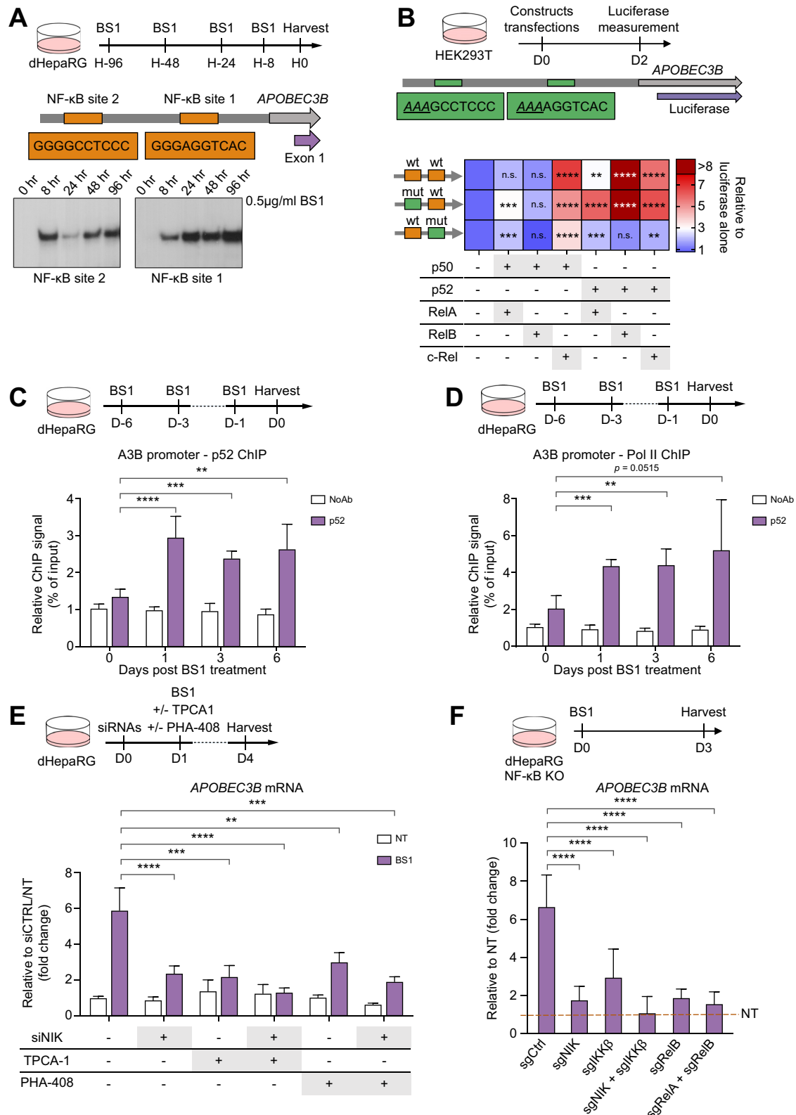
Fig. 1. Lymphotoxin beta receptor agonisation induces APOBEC3B through NF- \kappa B signalling. (A) dHepaRG were treated for indicated times with 0.5 \mu g/ml BS1. Upper panel: schematic representation of the experiment. Lower panel: labelled probes containing the NF- \kappa B binding sites were analysed by EMSA. (B) HEK293T cells were co-transfected with a luciferase construct containing APOBEC3B promoter (-230, +18, distance to transcription start site) wt or mutated for each NF- \kappa B binding sites, together with NF- \kappa B-transcription-factors-expressing plasmids. Upper panel: schematic representation of the experiment. Lower panel: schematic representation of the downstream promoter region with the inserted mutations of the NF- \kappa B sites. Luciferase activity was assessed 48 h post-transfection. Heat map represents the mean of 1 experiment performed in triplicate. (C,D) dHepaRG were treated for the indicated time with 0.5 \mu g/ml BS1.
