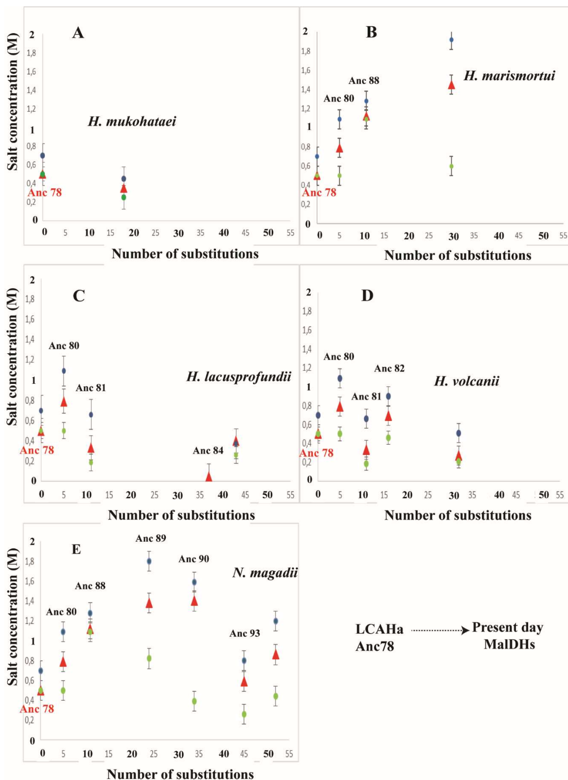
FIG. 3. Evolution of the conformational stability of ancestral and extant halobacterial MalDHs. The M_{f/2}^f values (y-axis) are plotted against the number of amino acid replacements accumulated since the LCAHa Anc78 MalDH (x-axis). Values were recorded in KCl (red), CsCl (blue) and KF (green). (A and B) evolutionary path leading to two extant MalDH enzymes of group A species, H. muko and H. mari MalDHs respectively. (C and D) evolutionary path leading to two extant MalDH
