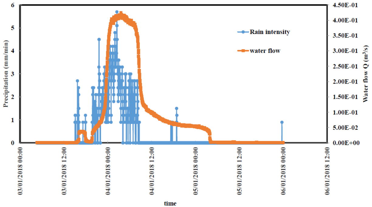
Fig.4. Rain intensity and water fluxes at the basin inlet during the rainy episode from January 3 to January 6, 2018.
