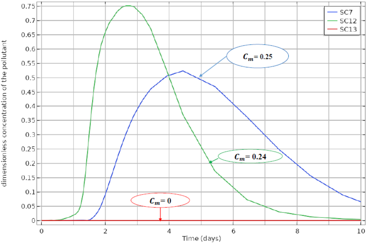
Fig.11. Effect of piezometers location on the estimate of pollutant fluxes
