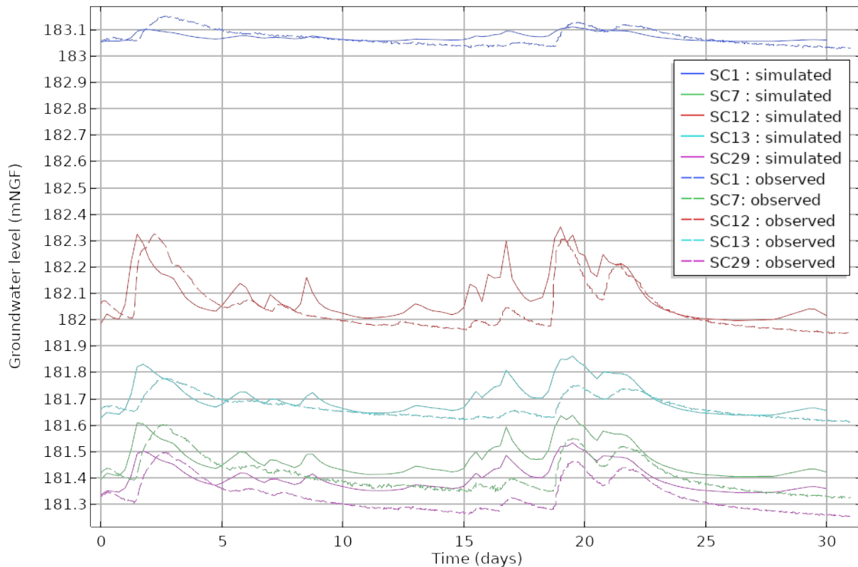
Fig.8. Comparison of piezometric levels between observed and simulated observation points during the month of December 2018
