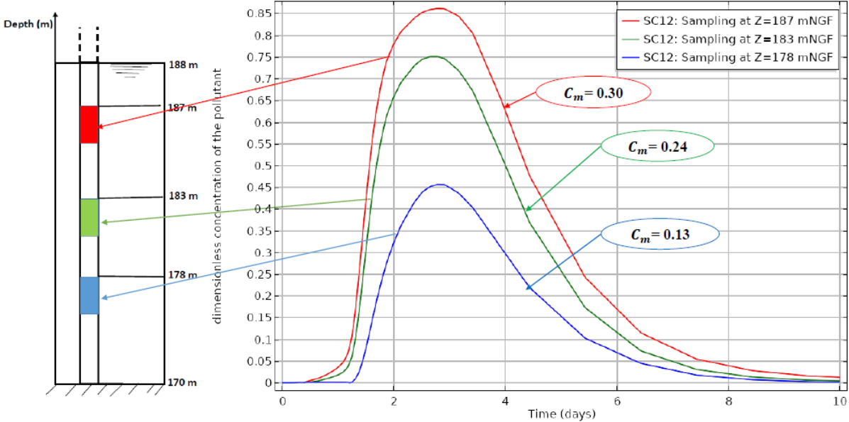
Fig.12. Effect of integrative sampler depth in the piezometer SC12 on the estimate of pollutant concentration
