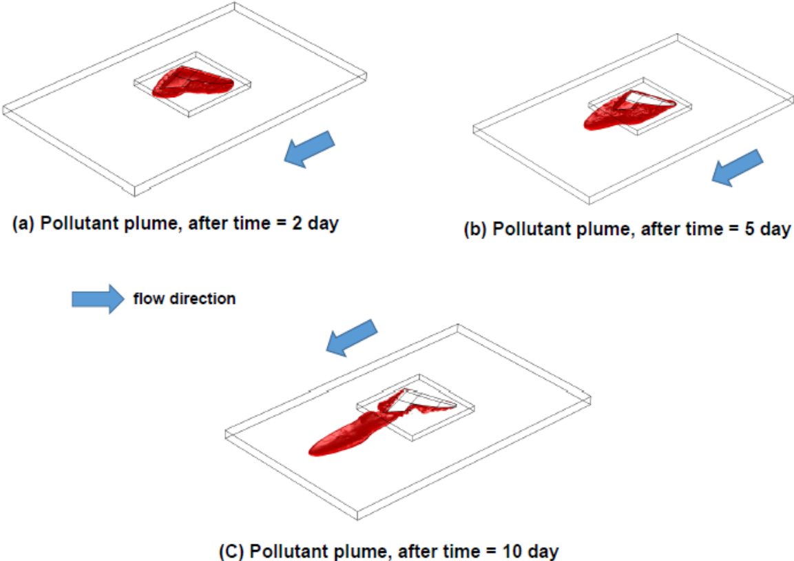
Fig.10. Evolution of the pollutant plume (isovalues at c = 0.2 ) during the infiltration-drainage process
