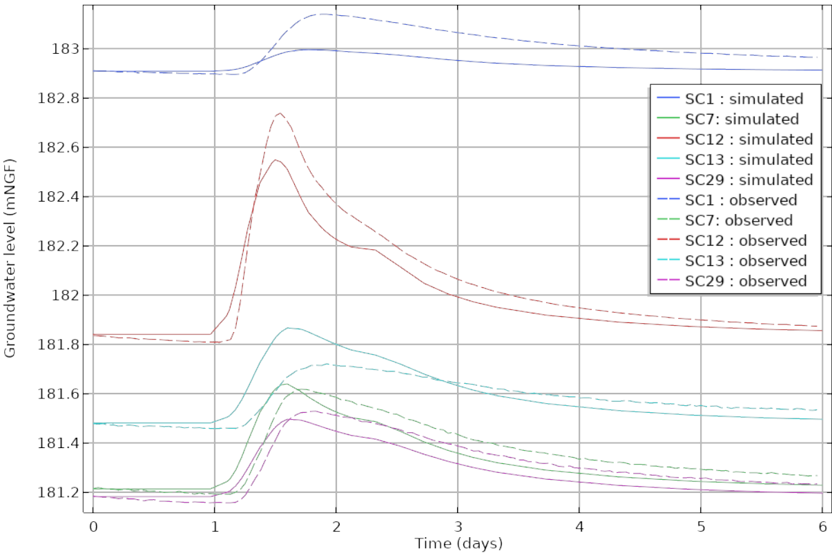
Fig.5. Comparison of piezometric levels between observed and simulated observation points during the rainy episode from January 3 to January 6, 2018.
