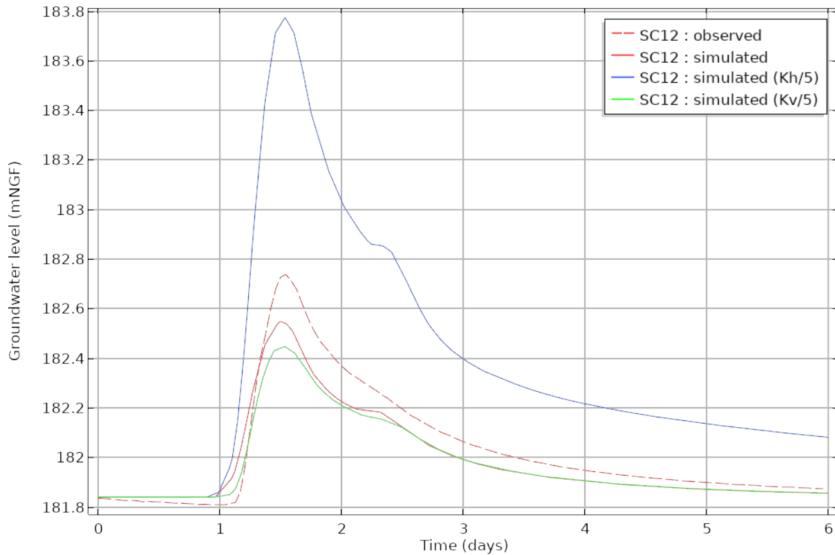
Fig.6. Influence of permeability on the piezometric levels (rainy episode from January 3 to January 6, 2018).
