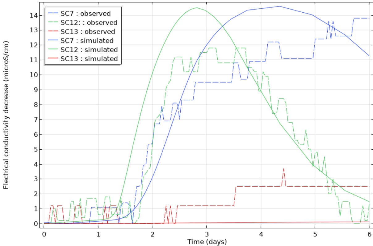
Fig.9. Comparison of electrical conductivity decrease between observed and simulated observation points during the rainy episode from January 3 to January 6, 2018.
