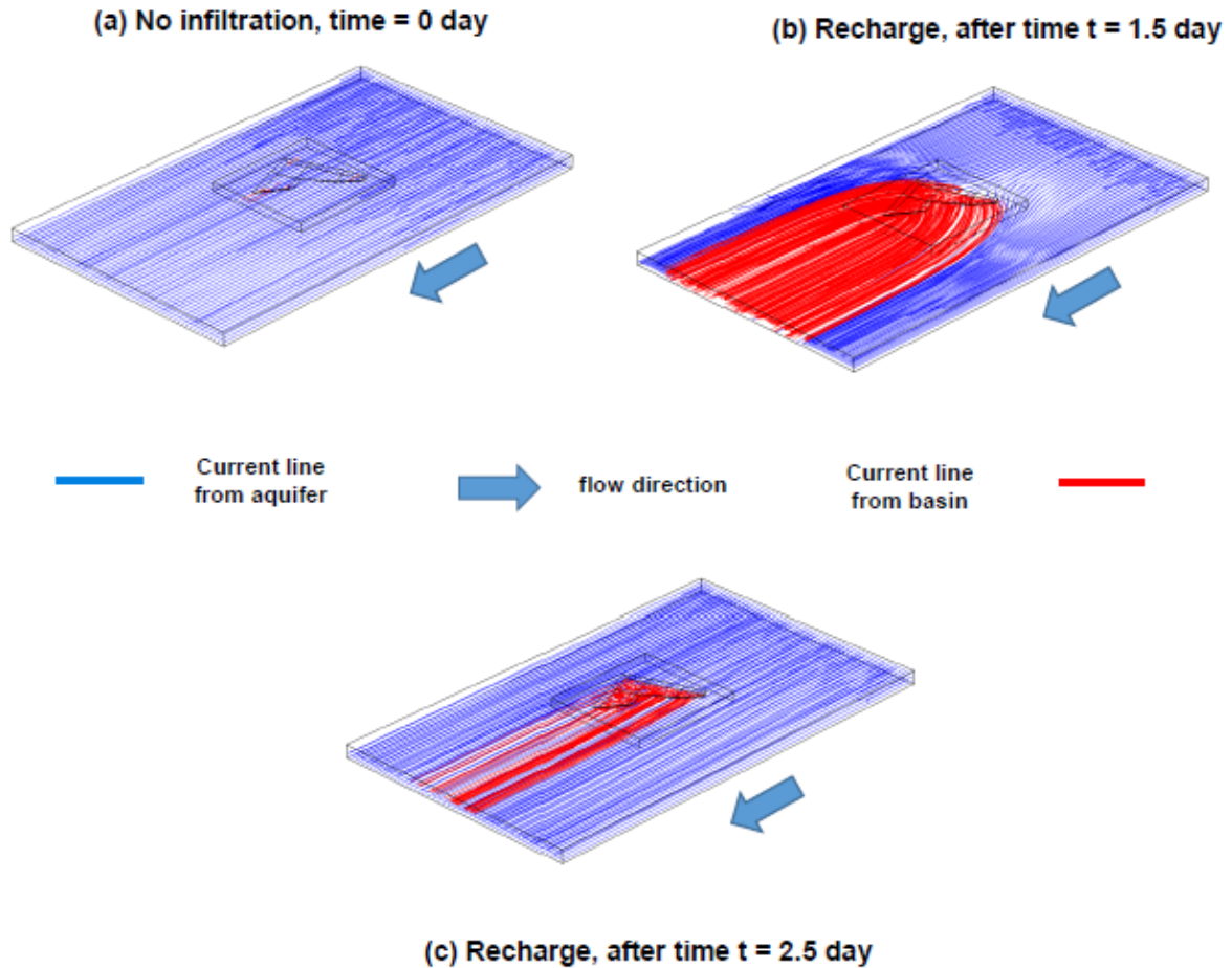
Fig.7. The current lines during the simulation of the reference rainy episode (image (a) corresponding to zero recharge, image (b) to 1.5-day period of recharge and image (c) to 2.5-day period of recharge).
