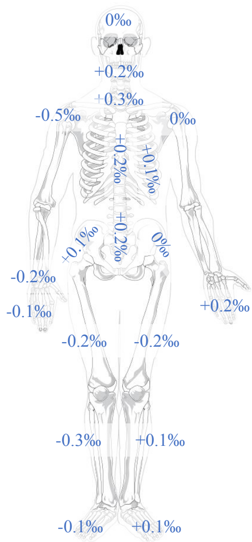
TG-01 Mean \delta^{18}\text{O}_p (V-SMOW): 16.6‰ Standard Deviation: 0.2‰
