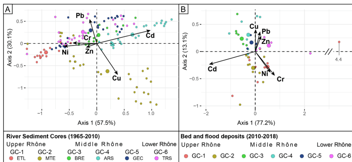
Fig. 4. Principal Component Analyses (PCA-biplots) performed separately for (A) samples from river sediment cores ( n = 137 ) and (B) for bed and flood deposit samples ( n = 78 ). GC refers to the geographical clusters defined in the text. The bigger circles are the centroids of the data.
