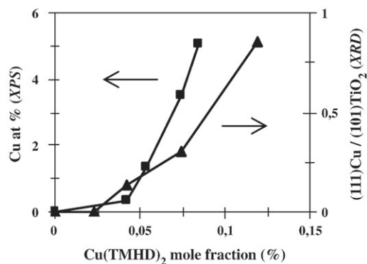
Fig. 7. Variation of the Cu content in the films determined by XPS (at.%, left axis) and ratio of (111) Cu/(101) \text{TiO}_2 XRD intensity (right axis, \theta - 2\theta configuration) as a function of the \text{Cu}(\text{TMHD})_2 mole fraction in the input gas phase.
