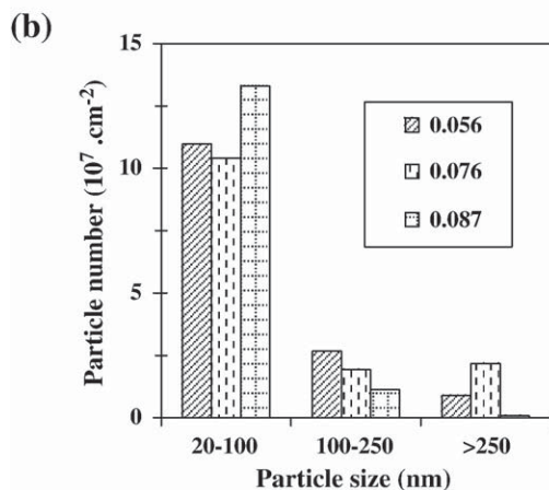
Fig. 9. TEM micrograph of a TiO 2 -Cu film deposited at 683 K directly on a microscopy grid made of amorphous carbon (a) and size distribution of the density of particles for different mole fractions of Cu(TMHD) 2 in the gas phase (b): 0.056%, 0.076% and 0.087%.
