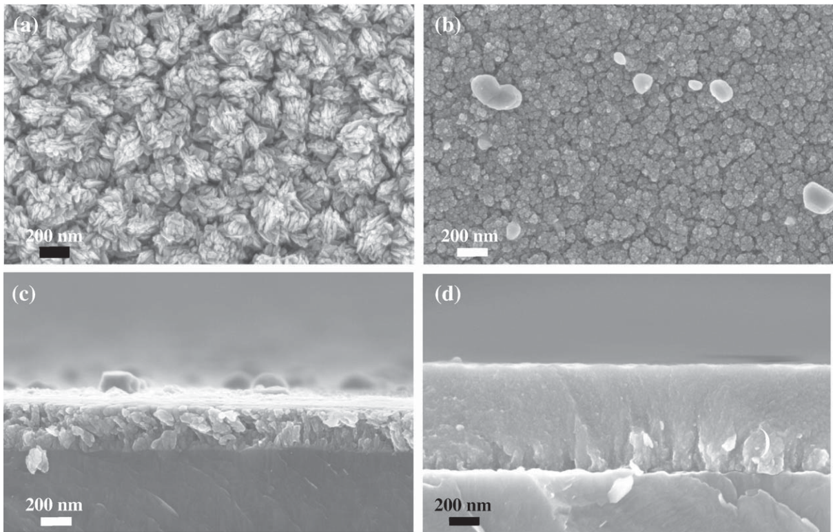
Fig. 2. FEG-SEM micrographs of TiO 2 -Cu films deposited on silicon wafer as a function of the Cu(TMHD) 2 mole fraction in the reactive gas phase: (a) 0% at 683 K (pure TiO 2 ); (b) 0.076% at 683 K (surface morphology); (c) 0.076% at 683 K (cross section); (d) 0.076% at 623 K (cross section). The scale bar is the same for each micrograph.
