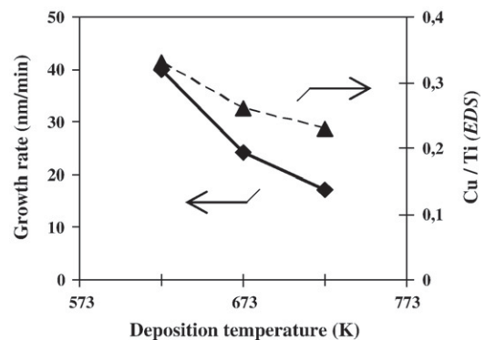
Fig. 4. Influence of the growth temperature on the deposition rate and on the content of copper in TiO 2 -Cu films (EDX analyses).
