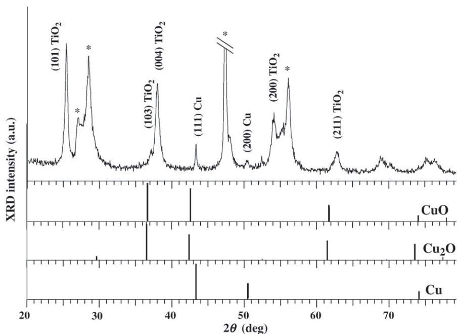
Fig. 5. Grazing angle XRD pattern of a \text{TiO}_2 -Cu film showing the presence of anatase and metallic copper. Peaks noted with an asterisk originate from the substrate.
