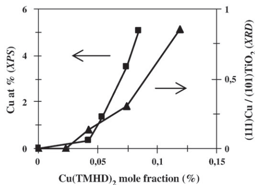
Fig. 7. Variation of the Cu content in the films determined by XPS (at.%, left axis) and ratio of (111) Cu/(101) \text{TiO}_2 XRD intensity (right axis, \theta -2 \theta configuration) as a function of the \text{Cu}(\text{TMHD})_2 mole fraction in the input gas phase.
