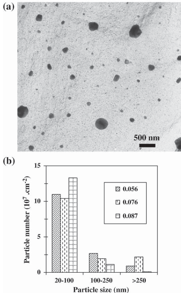
Fig. 9. TEM micrograph of a TiO 2 -Cu film deposited at 683 K directly on a microscopy grid made of amorphous carbon (a) and size distribution of the density of particles for different mole fractions of Cu(TMHD) 2 in the gas phase (b): 0.056%, 0.076% and 0.087%.
