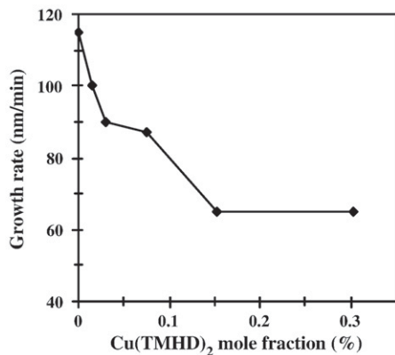
Fig. 3. Influence of the Cu(TMHD) 2 mole fraction on the growth rate of TiO 2 -Cu films (T=683 K).
