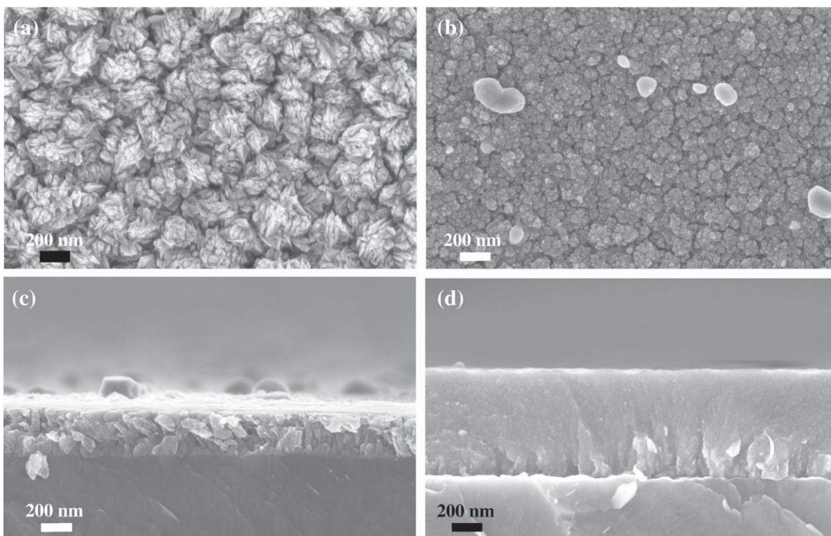
Fig. 2. FEG-SEM micrographs of \text{TiO}_2 -Cu films deposited on silicon wafer as a function of the \text{Cu}(\text{TMHD})_2 mole fraction in the reactive gas phase: (a) 0% at 683 K (pure \text{TiO}_2 ); (b) 0.076% at 683 K (surface morphology); (c) 0.076% at 683 K (cross section); (d) 0.076% at 623 K (cross section). The scale bar is the same for each micrograph.
