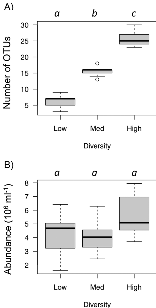
Figure 2. Preliminary tests results for initial bacterial diversity gradient and abundances. (A) Number of operational taxonomic units (OTUs) for the three bacterial diversity levels after the acclimation period (48 h of incubation in Thau lagoon water, Fig. 1C). Per diversity level, the three immigration treatments are combined (no immigration, 1% and 10% of immigration, n=9 ). Dilution rates are: low = 10^{-5} , Med = 10^{-3} and High = no dilution (see methods). (B) Bacterial abundance after the acclimation period for the three diversity treatments. The three immigration treatments are combined per diversity level. Diversity levels connected by the same letter are not significantly different (Tukey-Kramer test, p < 0.05 ). doi:10.1371/journal.pone.0037620.g002
