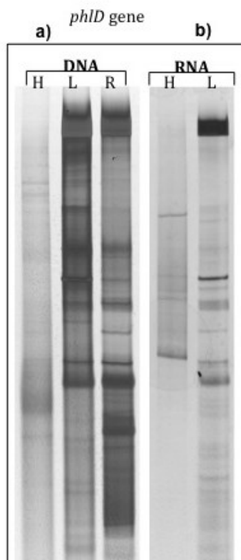
Figure 1. DGGE patterns of phlD gene fragments amplified from (a) heavy, light, and root DNA fractions and (b) 12 C- & 13 C-RNA fractions retrieved from the rhizosphere of A. thaliana after 27 days of 13 CO 2 labeling.
