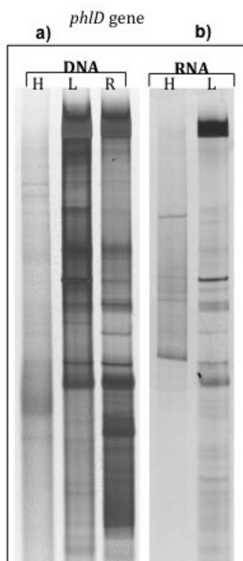
Figure 1. DGGE patterns of phlD gene fragments amplified from (a) heavy, light, and root DNA fractions and (b) ^{12}\text{C} - & ^{13}\text{C} -RNA fractions retrieved from the rhizosphere of A. thaliana after 27 days of ^{13}\text{CO}_2 labeling.
