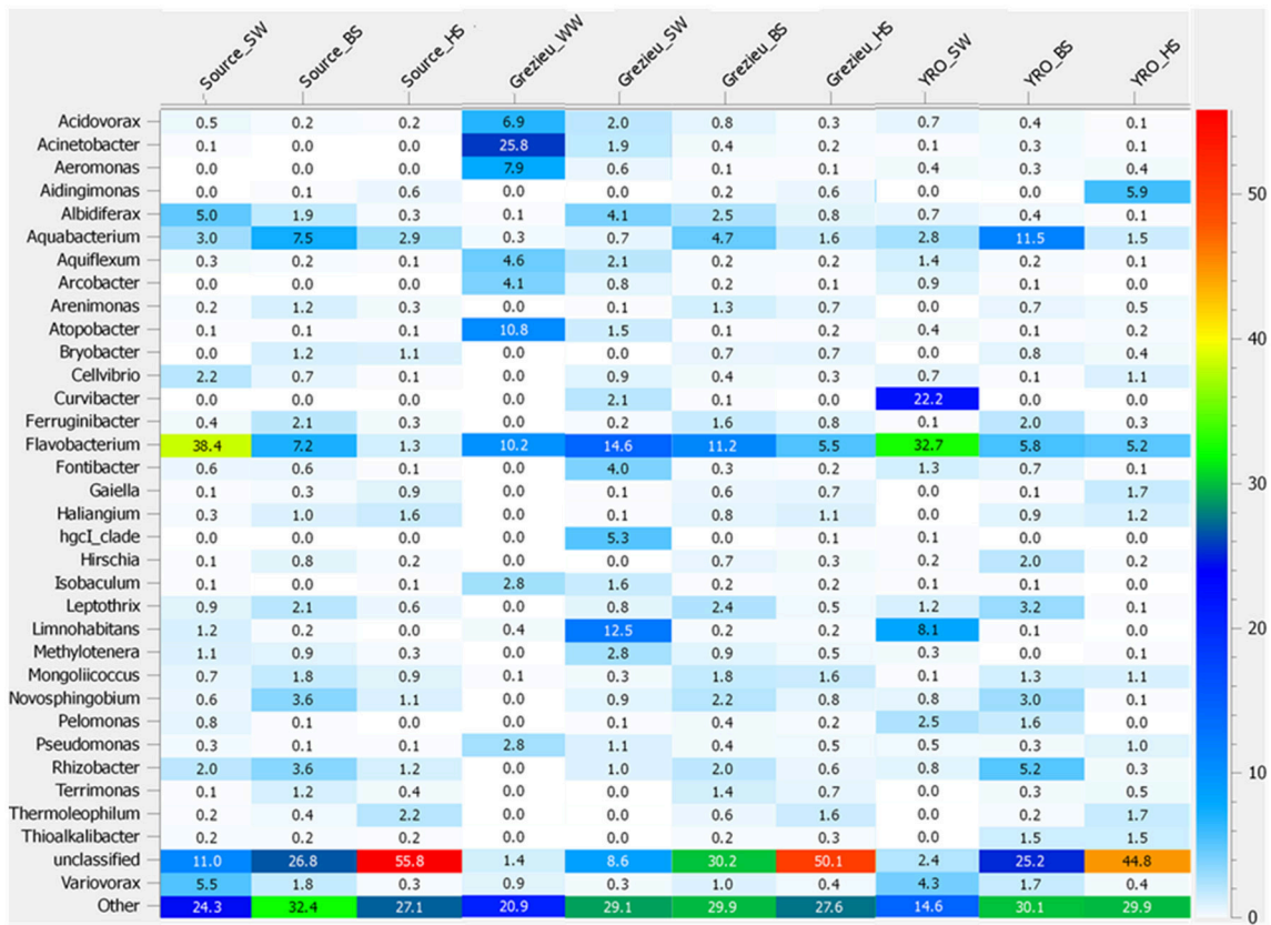
FIGURE 4 | Heatmap illustrating the significance of some genera inferred from the 16S rRNA gene dataset recovered from river and wastewater samples. The 50K dataset (5670 reads per sample) containing 16S rRNA gene sequences from surface waters (SW), benthic (BS), and hyporheic sediments (HS), and wastewater (WW), sampled along the Chaudanne river, were used (see text). Genera representing less than 0.4% of the full dataset were merged and grouped into the term “Other.”
