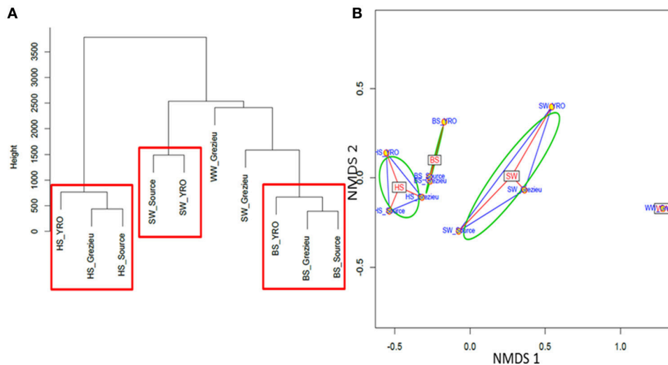
FIGURE 5 | Ascendant Hierarchical Classification (A) and Non Metric Multi-Dimensional Scaling (B) analyses of 16S rRNA gene OTU. The 50K dataset (5670 reads per sample) containing 16S rRNA gene sequences from surface waters (SW), benthic (BS), and hyporheic sediments (HS), and wastewater (WW), sampled along the Chaudanne river was used (see text). Vertical lines in (A) are indicative of the proximity between the OTU distribution patterns.
