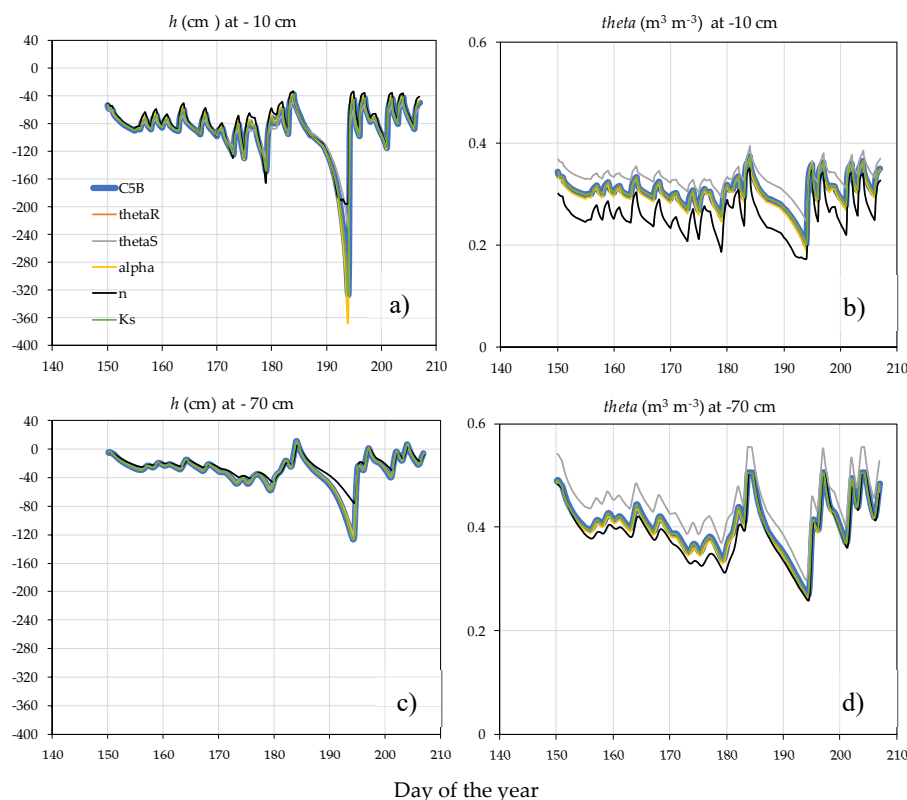
Figure 9. Temporal trend of soil pressure head (a,c) and soil water content (b,d) obtained by perturbing the van Genuchten parameters under the C5 approach.
