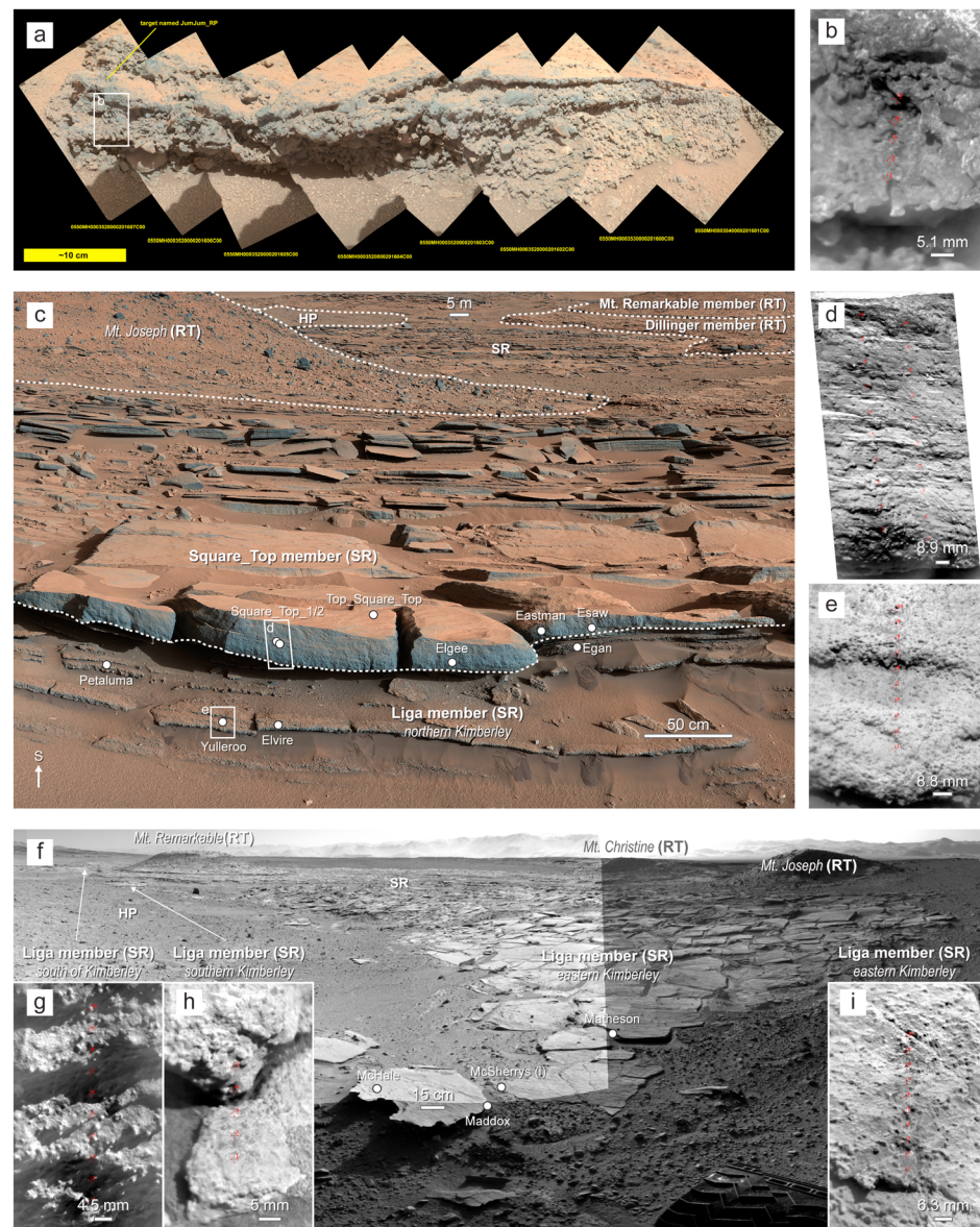
Figure 4. Facies of the lowermost members of the Kimberley formation: the Point_Coulomb, Liga, and Square Top members. (a) Mosaic of MAHLI images of the “Bungle Bungle” outcrop, in Violet Valley of the Point_Coulomb member; this is the site of the Jum_Jum target. (b) ChemCam RMI image of Jum_Jum (RMI images: CR0_446313251PRC_F0271004CCAM01550L2, CR0_446313840PRC_F0271004CCAM01550L2). (c) Mastcam panorama (mcam02407.0000b.kimberley_16x1_L0_41 x 6_L0_R0) of northern Kimberley showing the Liga and Square_Top members in the foreground and the Dillinger and Mount Remarkable members in the background. ChemCam bedrock targets of northern Kimberley are indicated by white dots. (d) ChemCam RMI images of the targets Square_Top and Square_Top_2 (RMI images: CR0_448625272PRC_F0300740CCAM01576L1, CR0_448625586PRC_F0300740CCAM01576L1, CR0_448625872PRC_F0300740CCAM01576L1, CR0_448626158PRC_F0300740CCAM01576L1, CR0_448626444PRC_F0300740CCAM01576L1, CR0_448626723PRC_F0300740CCAM01576L1, CR0_448894050PRC_F0300740CCAM04578L1, CR0_448894336PRC_F0300740CCAM04578L1, CR0_448894623PRC_F0300740CCAM04578L1, CR0_448894910PRC_F0300740CCAM04578L1, CR0_448895202PRC_F0300740CCAM04578L1, and CR0_448895482PRC_F0300740CCAM04578L1). (e) ChemCam RMI images of Yulleroo target (RMI images: CR0_448892557PRC_F0300740CCAM03578L1 and CR0_448893154PRC_F0300740CCAM03578L2). (f) View to the WSW of Kimberley showing the Liga member (outcrops of eastern, southern, and south of Kimberley, Navcam panorama). ChemCam bedrock targets of eastern Kimberley are indicated by white dots. (g) ChemCam RMI images of the Moogana target (RMI images: CR0_453603301PRC_F0320000CCAM01632L2, CR0_453603673PRC_F0320000CCAM01632L2, CR0_453604023PRC_F0320000CCAM01632L2, and CR0_453604432PRC_F0320000CCAM01632L1). (h) ChemCam RMI images of the Harms target (RMI images: CR0_450840163PRC_F0310724CCAM02601L1 and CR0_450840630PRC_F0310724CCAM02601L1). (i) ChemCam RMI images of the McSherrys target (RMI images: CR0_450222702PRC_F0310216CCAM02594L1, CR0_450223041PRC_F0310216CCAM02594L1, CR0_450223381PRC_F0310216CCAM02594L1, and CR0_450223381PRC_F0310216CCAM02594L1). ChemCam LIBS points are indicated (red) in Figure 4b, d, e, and g-i.
