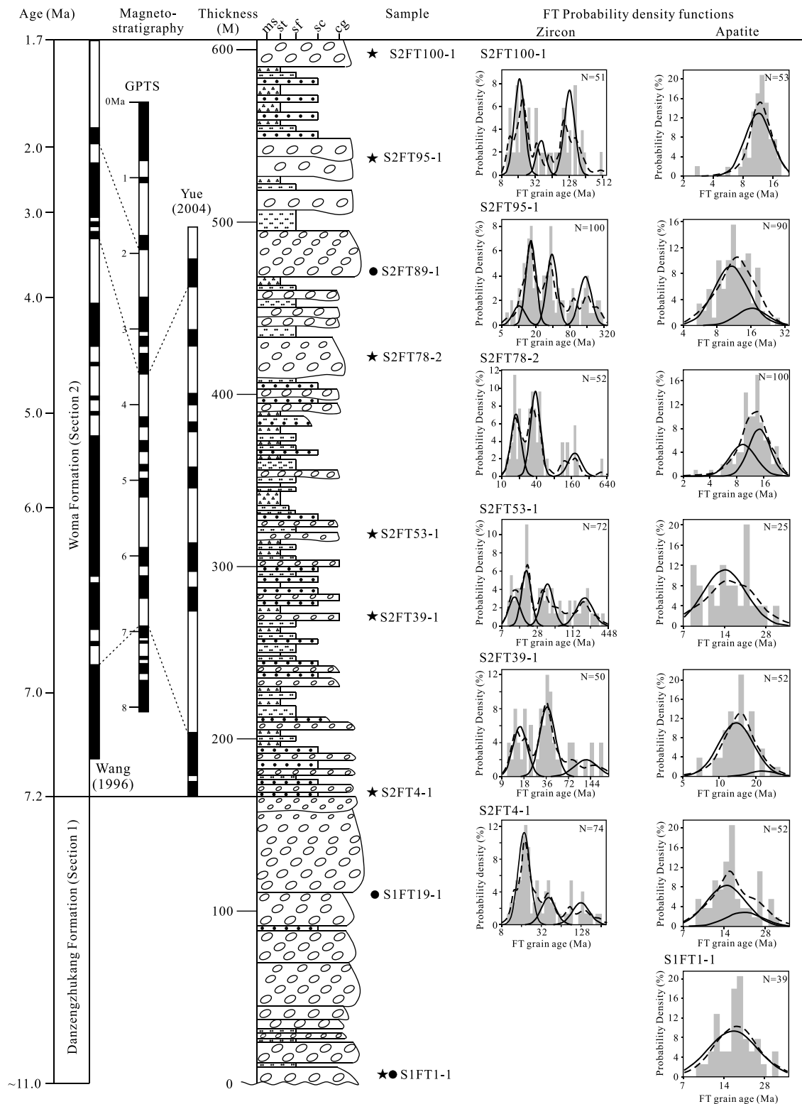
Figure 5. Stratigraphic column of the late Neogene sedimentary fill of the Gyrong basin measured in the field and fission-track age distribution of the samples (shown as histograms and probability density curves with fitted age populations). Lithology codes: ms, mudstone; st, siltstone; sf, fine sandstone; sc, coarse sandstone; and cg, conglomerate. GPTS: Geomagnetic Polarity Timescale [Cande and Kent, 1995], magnetotransigraphy data from Wang et al. [1996] and Yue et al. [2004]. Circle, zircon U-Pb sample and star, fission-track sample. Probability density functions and age populations for fission-track data are calculated using BinomFit [Brandon, 1992, 1996]. The dashed line is the single-grain age probability density function of the entire population; solid lines are modeled probability density functions for the fitted age populations; N is the number of dated grains. Detailed plots are shown in the supporting information (Figures S1 to S3).
