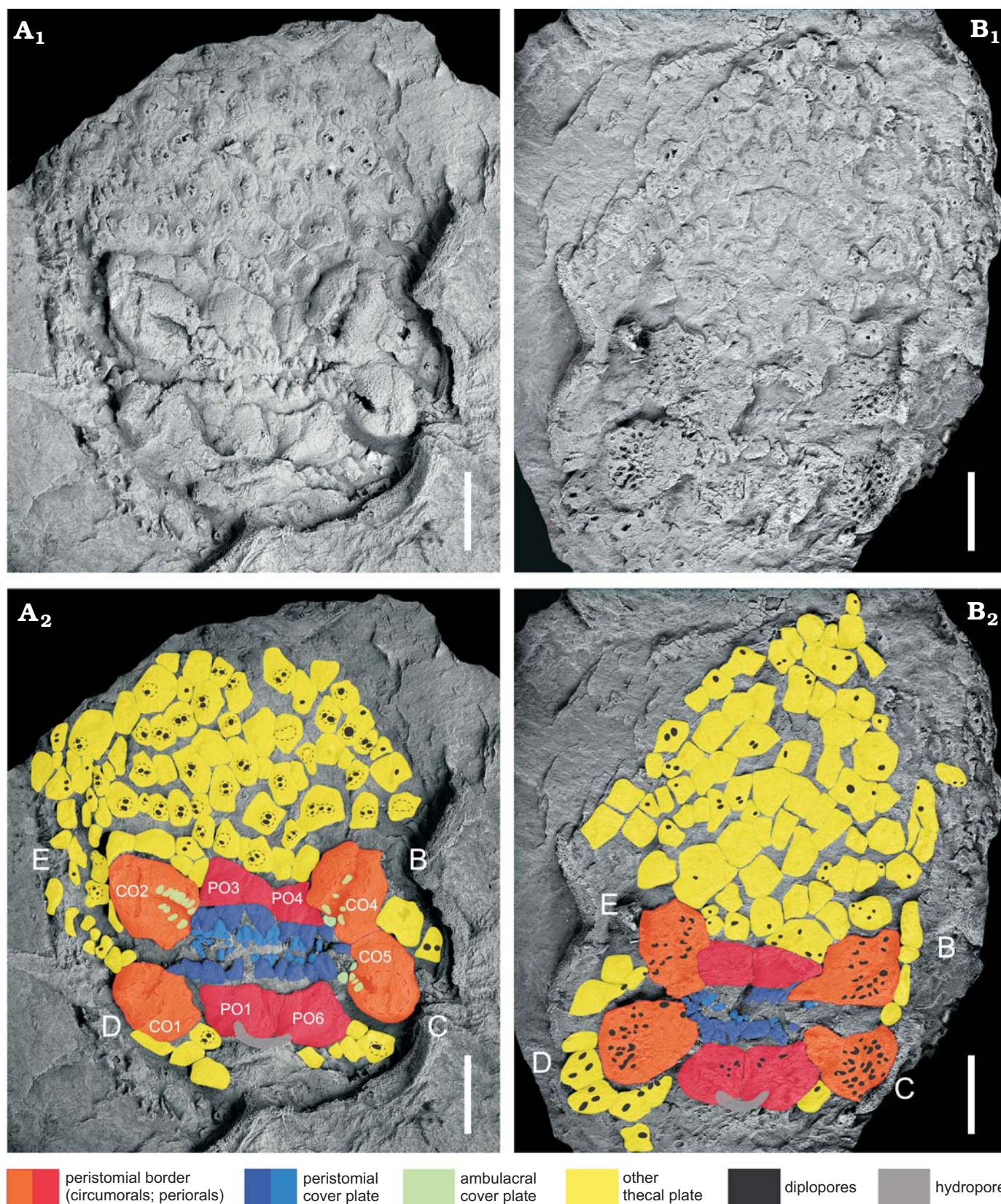
Fig. 6. Oral surface of the diploporite blastozoan Lepidocalix pulcher Termier and Termier, 1950a (MUA. 1024020); Middle Ordovician, Stita, Algeria. A. Four peri-orals (PO1, PO3, PO4, and PO6) between four circum-orals (CO1, CO2, CO4, and CO5), peristome partially covered by small subtriangular oral cover plates biseries, diplopore-bearing polygonal thecal plates immediately surrounding the peristome, hydropore over PO1 and PO6; in external view. B. Surface showing numerous diploporos. Photographs (A 1 , B 1 ), coloured interpretations (A 2 , B 2 ) of both surfaces illustrating names using circum-orals and periorals (Paul 1973, 2017); in internal view. B–E ambulacral designations in Carpenter's system. Scale bars 5 mm.
