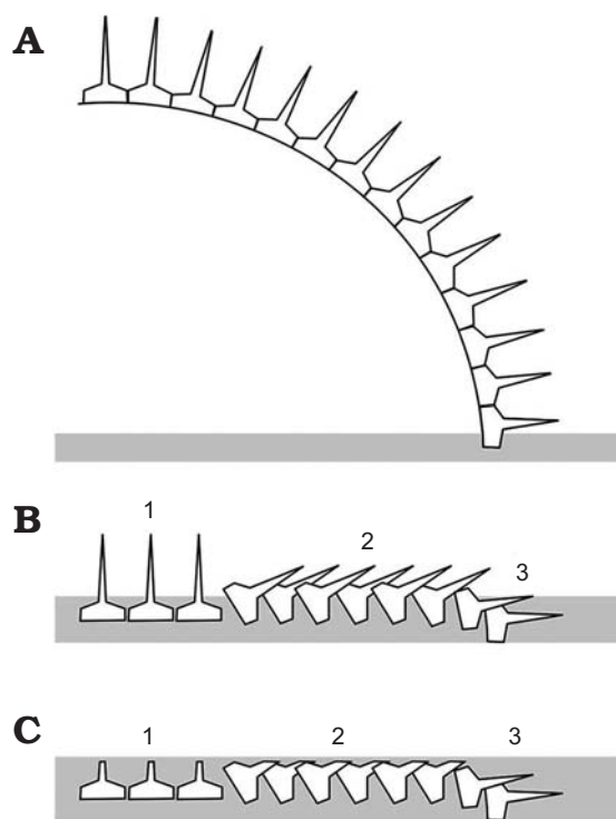
Fig. 7. Interpretation of taphonomy of the diploporite blastozoan Lepidocalix pulcher . A. Original disposition of partial theca still articulated. B. Positions of isolated plates after decay of ligaments and possible accumulation of a little more sediment (grey). Three areas can be distinguished. 1, areas where the spines were directed upwards in which the plate orientation has not changed significantly; 2, areas where the plates have rotated slightly so the spines rest on adjacent plates; 3, peripheral areas where the plates have again not rotated significantly, but the spines are buried in the sediment. C. Final stage of preservation in which parts of the plates not buried in sediment have been eroded, leaving plates in areas 1 and 2 lacking complete spines, those in area 2 apparently imbricate and spines only preserved in area 3.
