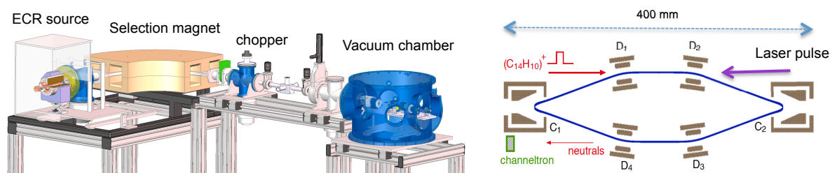
Fig.2 Experimental setup and the drawing of the Mini-Ring.
