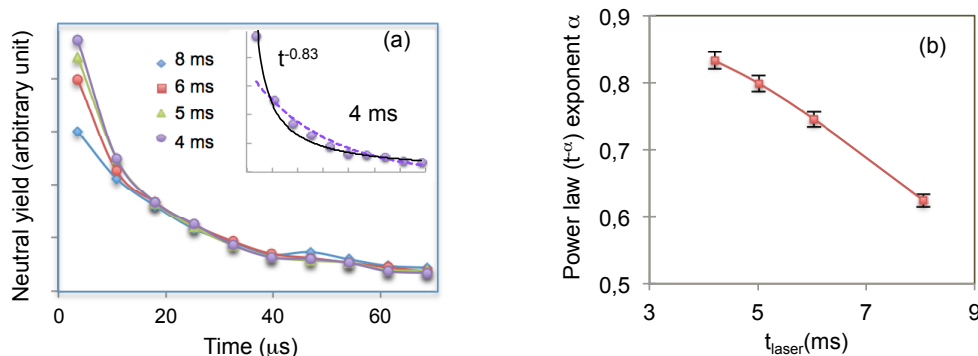
Fig.4 (a) Neutral yield as a function of time for the first 10 turns taking t_{\text{laser}} as time reference. Inset : Data for t_{\text{laser}} = 4 ms; Broken line: fit with an exponential function; solid line: fit with t^{-0.83} . (b) Power law exponent \alpha as a function of t_{\text{laser}} .
