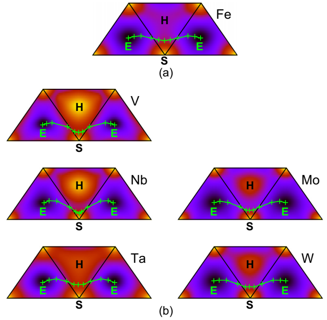
FIG. 10. (Color online) Projections of the 2D Peierls potentials in the (111) plane for (a) Fe and (b) nonmagnetic transition metals. Colors scale with energy going from the minimum (dark) to the maximum energy (light), which depends on the element considered. The dislocation trajectory from the cost function method along pathway (1) is shown in green (same as in Fig. 9).
