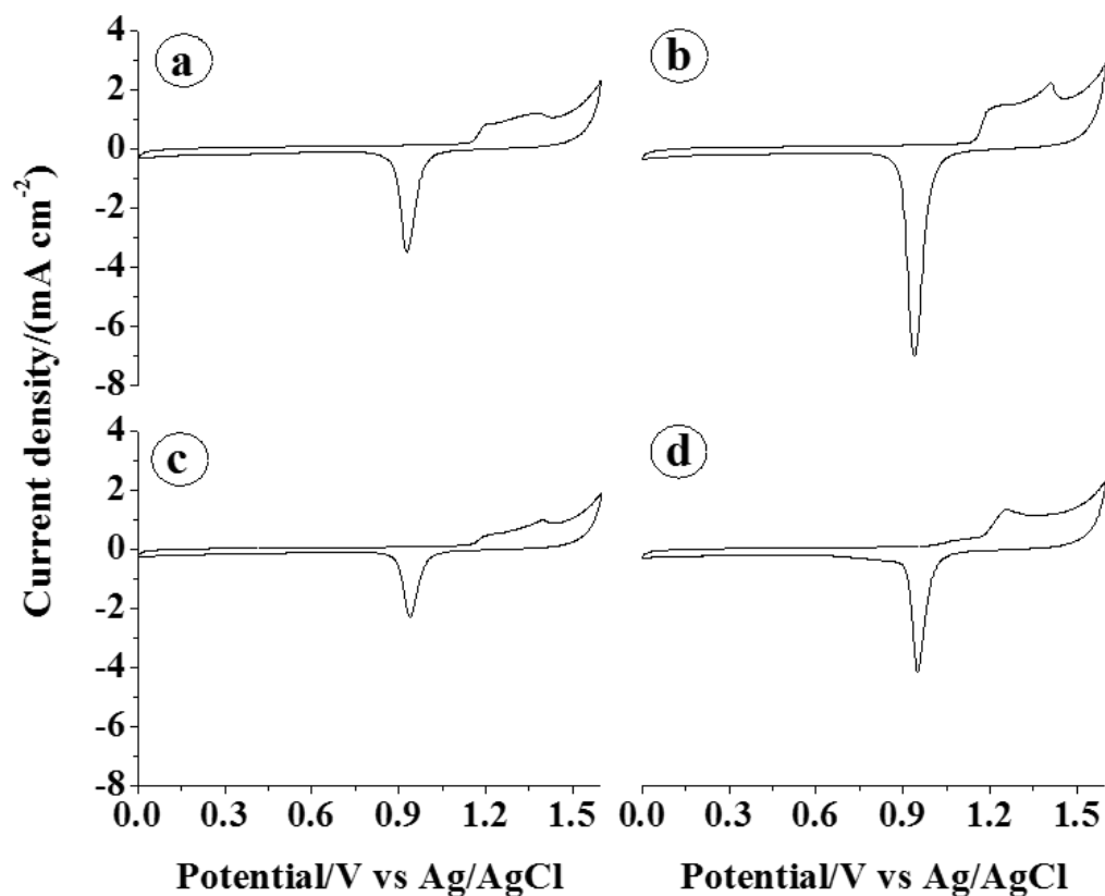
Figure 4. CV recorded with 50 \text{ mV s}^{-1} potential scan rate in a de-aerated solution of 0.5 \text{ M H}_2\text{SO}_4 at the various Au electrodes. (a) (\text{Au10kp})_{10\text{mT}} , (b) (\text{Au50kp})_{10\text{mT}} , (c) (\text{Au10kp})_{50\text{mT}} and (d) (\text{Au50kp})_{50\text{mT}} .
