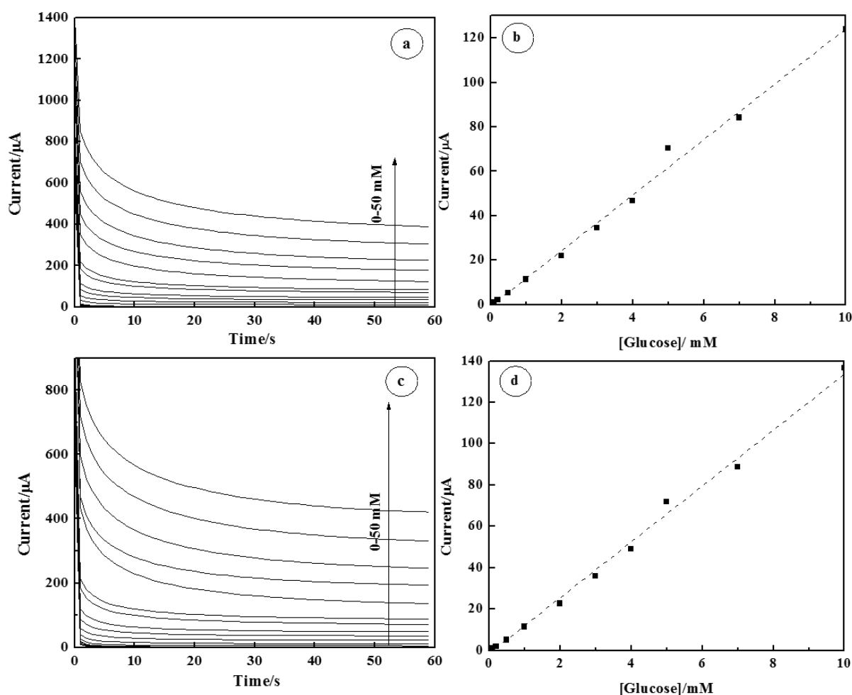
Figure 6. Chronoamperometry measurements recorded at the (Au50kp) 10mT electrode in argon-saturated 0.01 M PBS solution at pH 7.2 containing concentrations of glucose varying from 0 to 50 mM. (a) Chronoamperograms recorded at an applied potential of 0.25 V vs Ag/AgCl and (b) linearity domain. (c) Chronoamperograms recorded at an applied potential of 0.30 V vs Ag/AgCl and (d) linearity domain.
