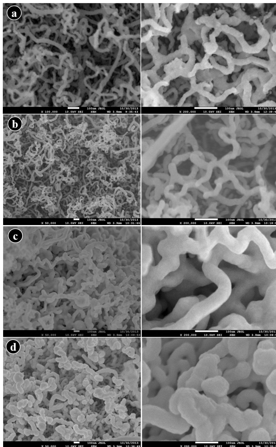
Figure 1. FESEM images of gold PLD-deposited onto carbon nanotubes in presence of oxygen: (a) (\text{Au}10\text{kp})_{10\text{mT}} , (b) (\text{Au}10\text{kp})_{50\text{mT}} , (c) (\text{Au}50\text{kp})_{10\text{mT}} and (d) (\text{Au}50\text{kp})_{50\text{mT}} .
