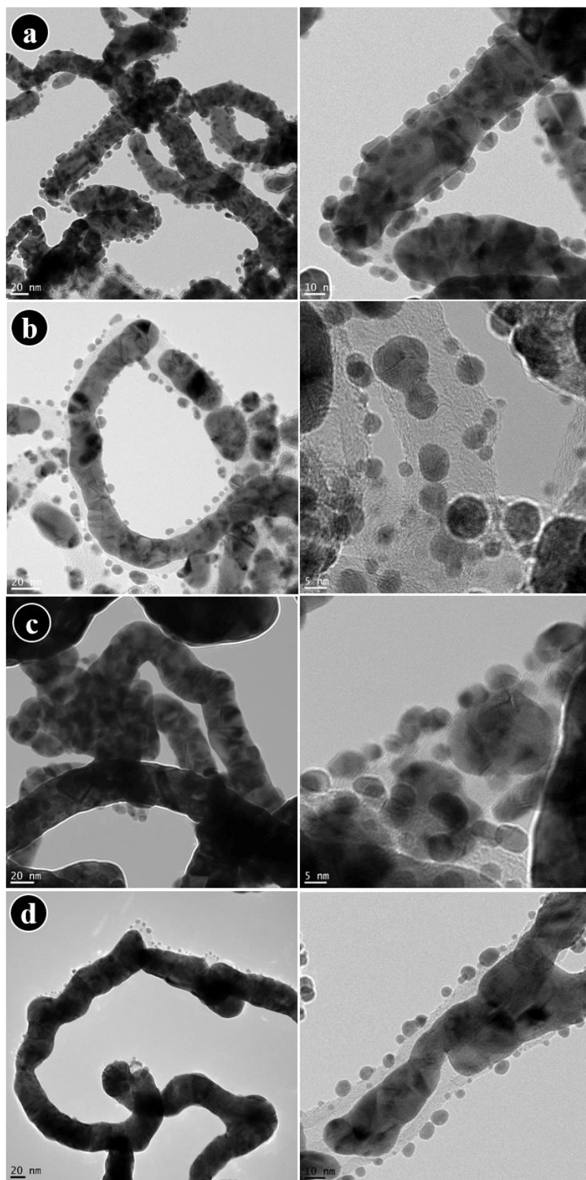
Figure 2. TEM and HR-TEM analyses of gold PLD-deposited onto carbon nanotubes in presence of oxygen: (a) (Au10kp) 10mT , (b) (Au10kp) 50mT , (c) (Au50kp) 10mT and (d) (Au50kp) 50mT .
