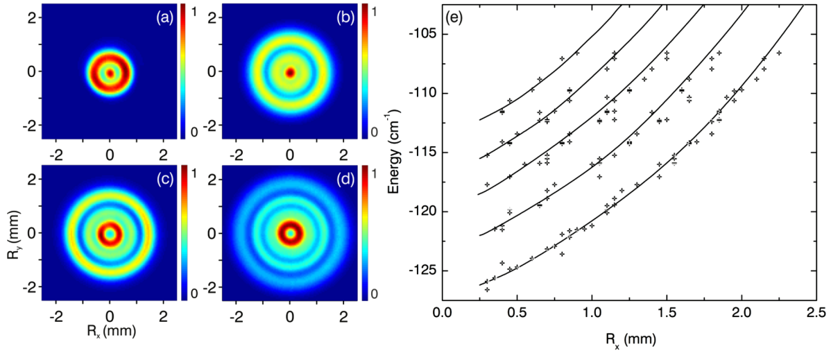
FIG. 2 (color online). Photoelectron images recorded for Stark states that decay via core-induced coupling to fast-ionizing red states. The examples shown in (a)–(d) are the (28, 22, 5, 0), (28, 25, 2, 0), (29, 21, 7, 0) and (21, 23, 5, 0) states, acquired at energies of -126.59 \text{ cm}^{-1} , -121.46 \text{ cm}^{-1} , -119.42 \text{ cm}^{-1} and -115.87 \text{ cm}^{-1} , respectively, in the presence of a 468 V/cm dc electric field. In all images, the intensities are normalized to the maximum occurring intensity. The main observation is that the number of interference minima increases smoothly as a function of energy. The interferences can be explained by considering the phase difference between different trajectories by which electrons can move from the ion to the detector. This is further illustrated in (e), where the positions of experimentally observed interference minima (+) are compared with semiclassically calculated positions (solid lines, using the method described in [19]).
