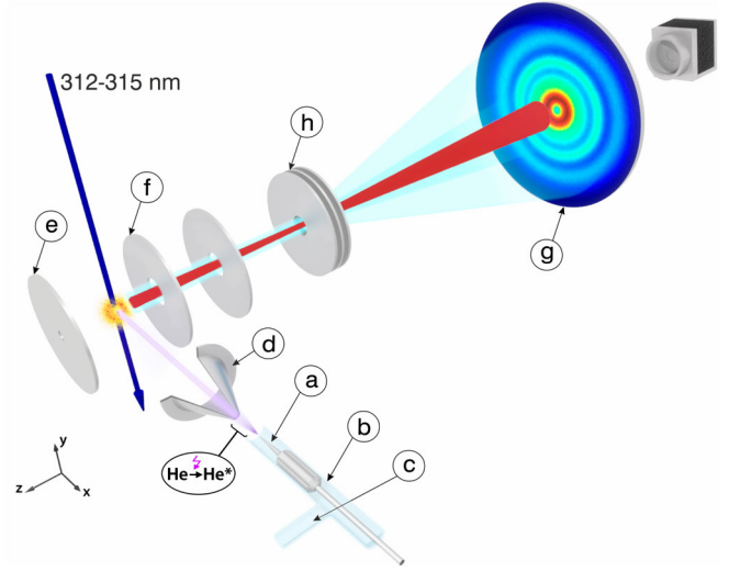
FIG. 1 (color online). Schematic representation of the experimental setup. Metastable 2^1\text{S} helium atoms are created by means of a dc electric discharge maintained between a Tantalum needle (a), surrounded by a quartz tube (b) and filled with He gas provided by a gas inlet (c), and a grounded skimmer (d). The ignition starts at -2 kV and is sustained at -0.7 kV and 20 mA. The \text{He}^* beam, formed by the skimmer ( \phi = 1 mm), crosses a tunable UV laser inside a velocity map imaging (VMI) spectrometer, permitting the excitation of quasibound Stark states that subsequently ionize. By applying a voltage difference across the repeller (e) and extractor (f) plates the photoelectrons are accelerated towards a position-sensitive detector (g) comprising 4-cm diameter MCP plates, a phosphor screen and a CCD camera. Halfway towards the detector, the photoelectrons pass through an Einzel lens (h), enabling magnification of the recorded photoelectron images by one order of magnitude.
