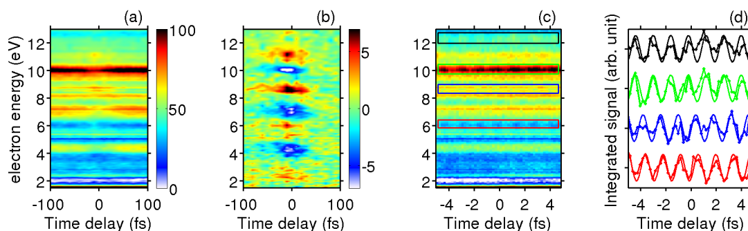
Figure 7. Time resolved photoelectron spectra of Naphthalene (XUV+IR) on the (a) femtosecond and on the (c) attosecond time scale. The modulation of the distribution of the map (a) is presented in (b) removing the static signal. The modulation of the distribution on the attosecond time scale is presented in (d) integrating a set of energetic range (indicated by rectangle of corresponding color in map (c)).
