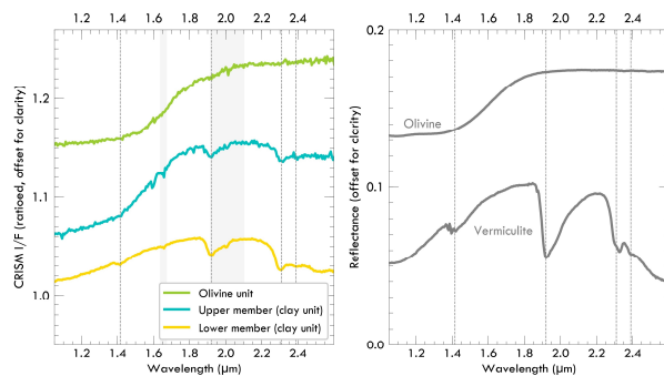
Figure 2. CRISM targeted spectra of three distinct members of the fractured unit compared to laboratory spectra of known minerals (CRISM Spectral Library).
