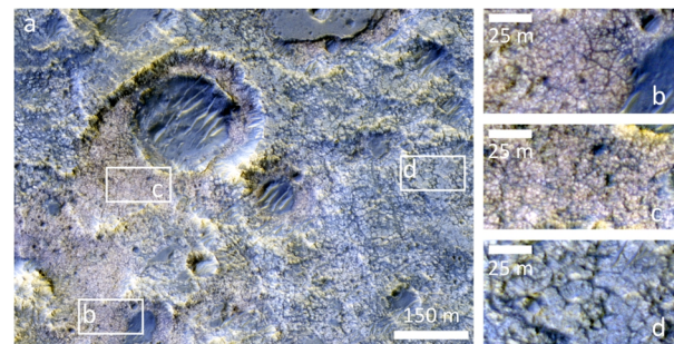
Figure 1. High resolution morphologies and color variations of the clay-bearing unit, as seen in HiRISE color (IR-RED-BG) ESP_045378_1980.
