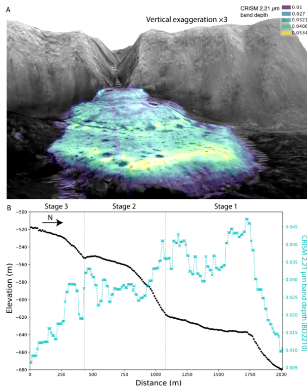
Figure 2. A) 3D rendering of an unnamed fan in Aeolis region with CRISM parameter map overlain on HiRISE image. The topography is exaggerated by 3 times. B) A cross-section along the fan direction of elevation profile (black) and extracted CRISM 2.21 \mu\text{m} band depth (cyan) corresponding to Si-OH or Al-OH absorptions.
