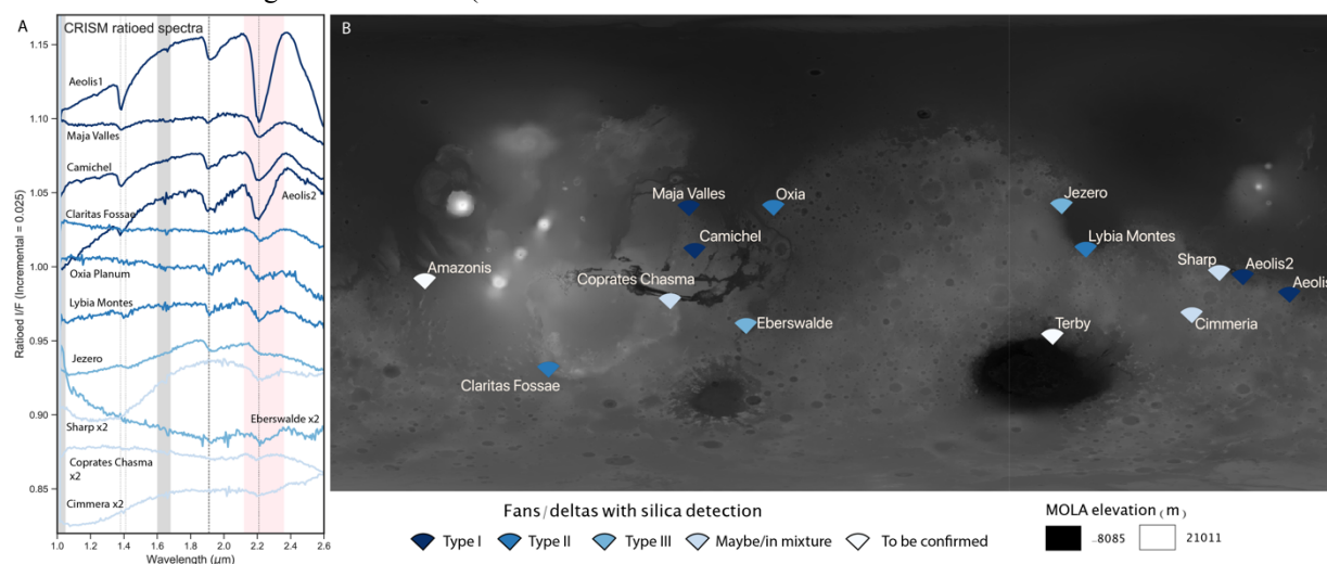
Figure 1. A) CRISM ratioed spectra of silica detections reported in previous literature associated with fans or deltas on Mars [5, 18-26], named after the closest named regions or features. The last four spectra are vertically exaggerated by 2 to show weak absorption features. The wide 2.21 \mu\text{m} bands of SiOH are marked by the pink shaded region. Dark grey shaded regions are known artifacts. B) Distribution of fans/deltas with silica globally. Symbols labeled with fan locations are overlain on the Mars Orbital Laser Altimeter (MOLA) topography.
