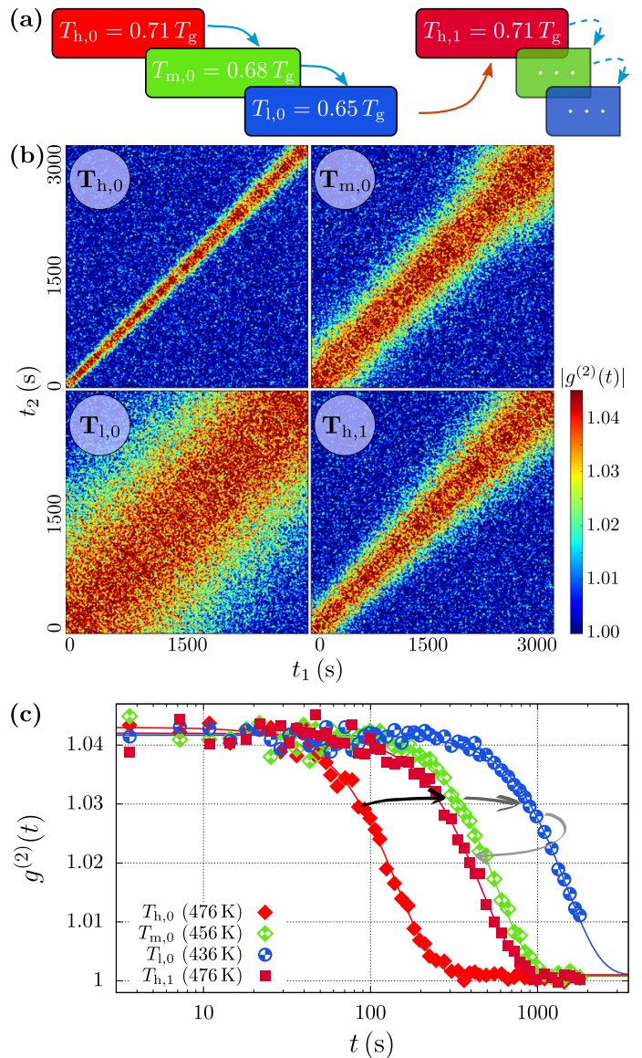
FIG. 1. (a) Scheme of applied temperature cycling. Relative temperatures are related to T_g of conventional \text{Cu}_{50}\text{Zr}_{50} MG. (b) TTFCs of UMG ap along first cycle in the T -protocol. Changes in the dynamics are signalled by different widths of the reddish area along the main diagonal. All TTFCs are equally scaled. (c) Corresponding g^{(2)}(q, t) , obtained by time-averaging over each TTFC from panel (b).
