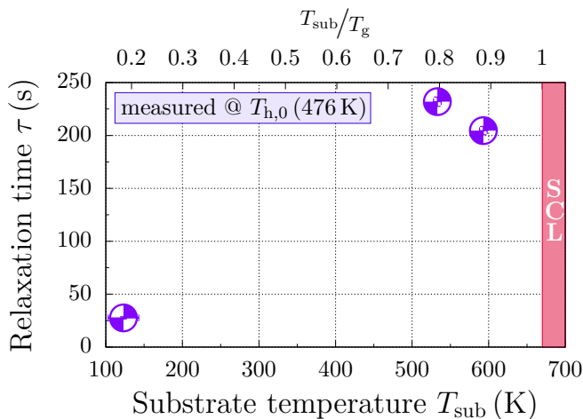
FIG. 4. Structural relaxation times measured at T_{h,0} for three \text{Cu}_{50}\text{Zr}_{50} films, prepared at different T_{\text{sub}} . Errorbars are within the symbol size. The red box indicates the supercooled liquid area with respect to T_g of the conventional MG.
