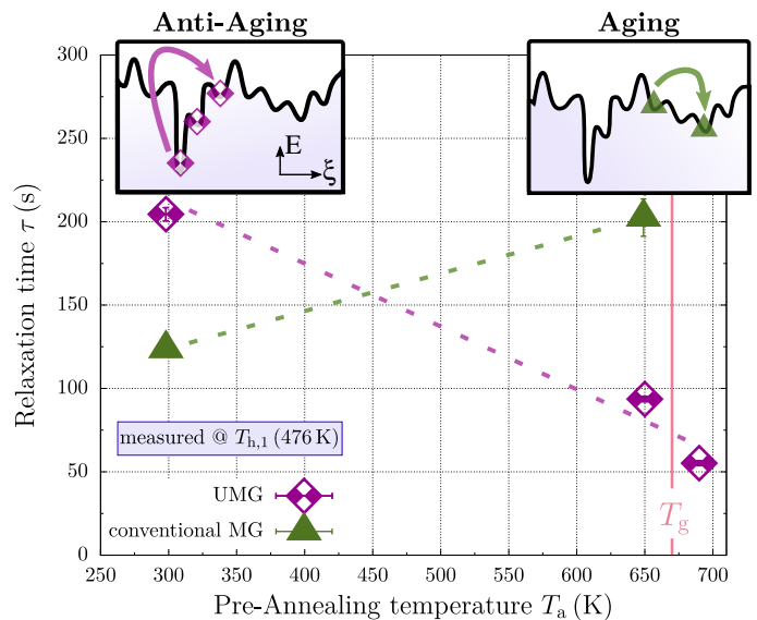
FIG. 3. Effect of pre-annealing temperature T_a on \tau for conventional \text{Cu}_{50}\text{Zr}_{50} MG (triangles) and UMG (open diamonds), measured at T_{\text{h},1} ( \hat{=} 476 K). The data at 298 K correspond to as-prepared samples. The vertical line depicts T_g of the conventional MG. The Anti-Aging of the UMG is indicated by the T_a -dependence which evolves inverse as normal aging. Dashed lines are a guide to the eye. Two insets depict a scheme of the data interpretation within the framework of the PEL.
