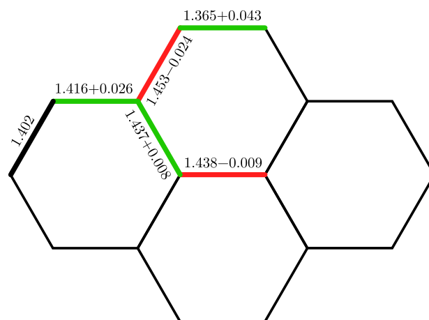
FIG. 7. Deformation in the S_1 state of pyrene as calculated with DFTB. Distances are given in Angstrom.
