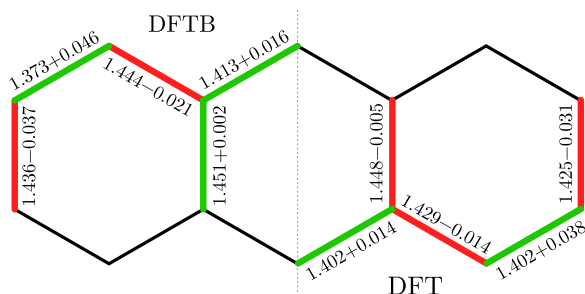
FIG. 3. Deformation in the S_1 state of anthracene calculated with DFTB (left) and DFT (right). Distances are given in Angstrom.
