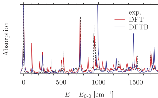
FIG. 14. Vibrationally resolved S_0 \rightarrow S_1 absorption spectrum of anisole. Vertical excitation energies are outside of the plotted spectral range. The experimental excitation spectrum from Ref. 46 has been scaled to match the intensity of the feature at 750 \text{ cm}^{-1} with the one calculated from DFT.
