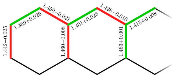
FIG. 5. Deformation in the S_1 state of pentacene as calculated with DFTB. Due to the symmetry of the deformation, only half of the molecule is shown. Distances are given in Angstrom.
