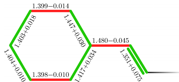
FIG. 12. Deformation in the S_1 state of trans -stilbene as calculated with DFTB. Distances are given in Angstrom.
