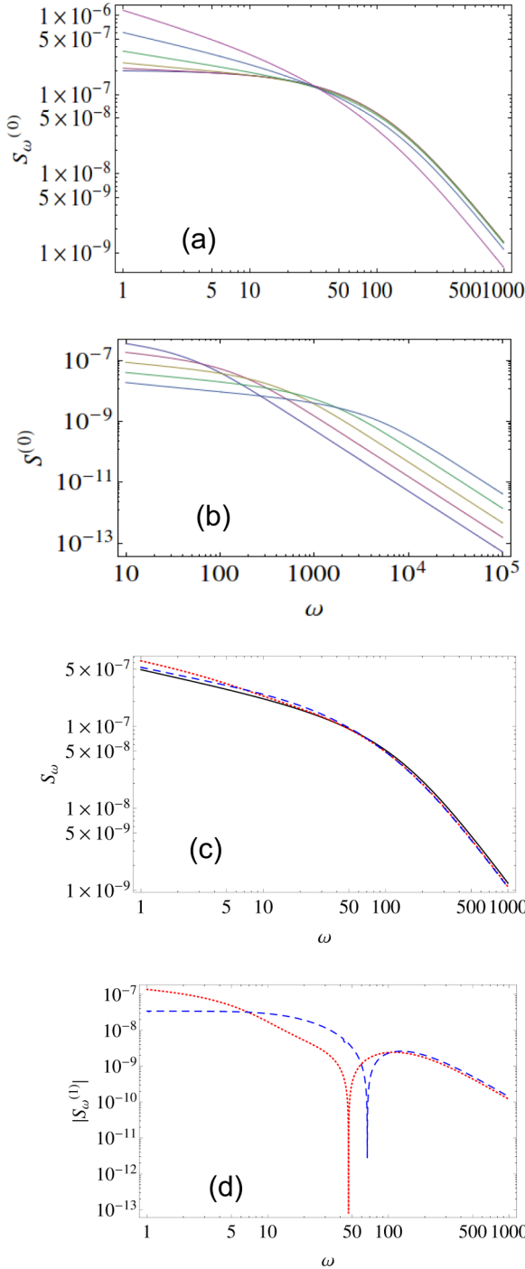
FIG. 3. SFSR spectrum \mathcal{S}_\omega as a function of \omega (in \text{s}^{-1} ). Parameters: \gamma = 20 \times 10^{-3} \text{ J m}^{-2} , R = 28 \text{ } \mu\text{m} , T = 298 \text{ K} , and \lambda = 632.8 \text{ nm} . (a) Flat substrate with \eta = 3.9 \text{ Pa s} , and various depths \bar{h}_s = 2^{-n} \times 500 \text{ } \mu\text{m} , with n = 0, \dots, 5 . The thick-dotted line corresponds to the limit \bar{h}_s = \infty , and the dotted line corresponds to the low-frequency limit Eq. (40) for n = 5 . (b) Flat substrate with \bar{h}_s = 100 \text{ } \mu\text{m} and \eta = 3^{-n} \text{ Pa s} with n = 0, \dots, 4 . (c) Substrate with parallel grooves of a sinusoidal cross section, with \bar{h}_s = 80 \text{ } \mu\text{m} , \delta h_s = 50 \text{ } \mu\text{m} , \lambda = 250 \text{ } \mu\text{m} , and \eta = 3.9 \text{ Pa s} . The dotted (red) and dashed (blue) lines are the spectra calculated over the maxima of the pattern for \phi_m = 0 and \pi/2 , respectively. The solid (black) line represents the spectrum of the flat substrate. (d) Absolute value of the first-order contribution |\mathcal{S}_\omega^{(1)}| , with the same parameters as in (c).
