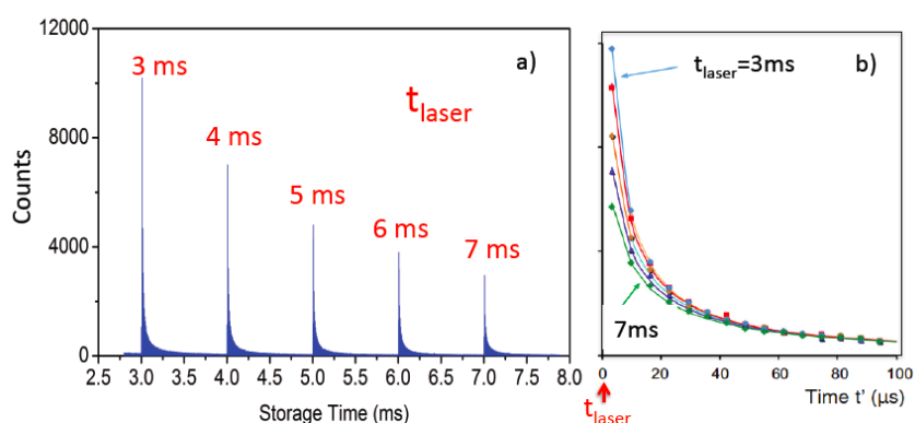
Fig.4 a) Neutral counts following laser pulse fired at t_{\text{laser}} from 3 to 7 ms. b) Neutral decay curves taking t_{\text{laser}} as time reference.
