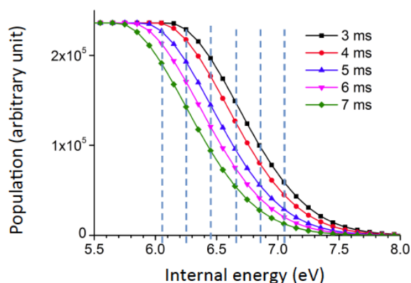
Fig.5 Population distributions simulated for t_{\text{laser}} from 3 to 7 ms. Crossing points with a vertical broken line give the population decay for each energy value.
