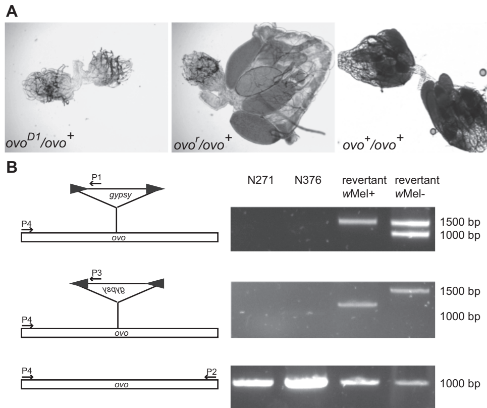
FIG 2 Ovaries of the progeny of an ovo D1 reversion test and detection of gypsy insertion into ovo by PCR. (A) Ovaries from a sterile ovo D1 /ovo + female, a revertant ovo I /ovo + female, and a wild-type ovo + /ovo + female shown by phase-contrast microscopy ( \times 50 magnification). (B) PCR detection of gypsy insertion into ovo in the two parental lines and samples of revertant F1 females. The schematic depicts the primers used (P1, P2, P3, and P4) and their localization in ovo and gypsy . Large arrows show gypsy long terminal repeats (LTR).
