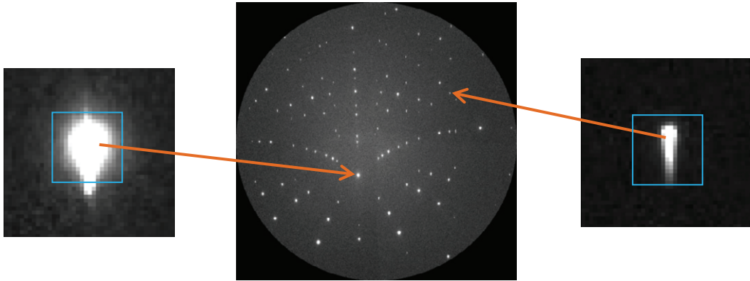
Fig. 1. Typical Laue pattern obtained on a Si single crystal. The blue squares represent the zone of interest (ZOI) around Laue spots (zoom) used for DIC.
