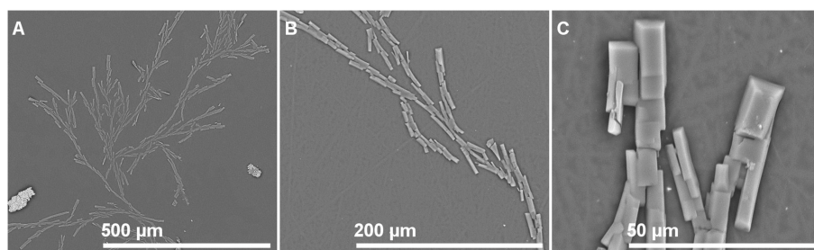
FIGURE 3 | LLDPE 2%: SEM observation of the film surface after aging (1 week at room temperature). Magnification from (A–C).
