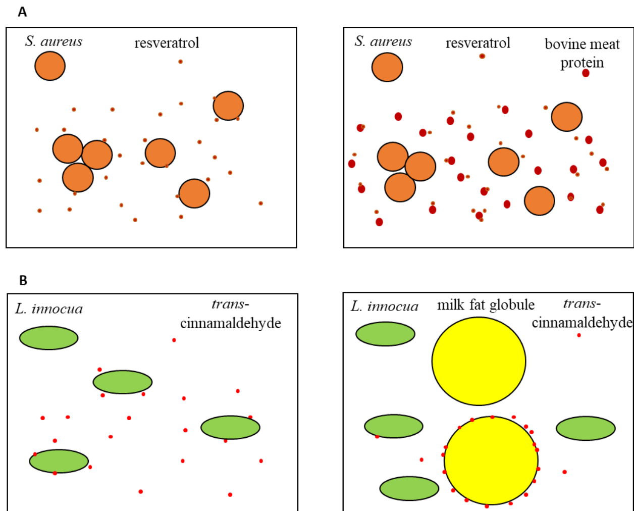
Figure 1. Scheme presenting interactions between resveratrol (as an example of polyphenol) and meat proteins (A) or between trans -cinnamaldehyde and milk fat globules (B) at the expense of interactions with S. aureus (A) or L. innocua (B) cells, respectively.
