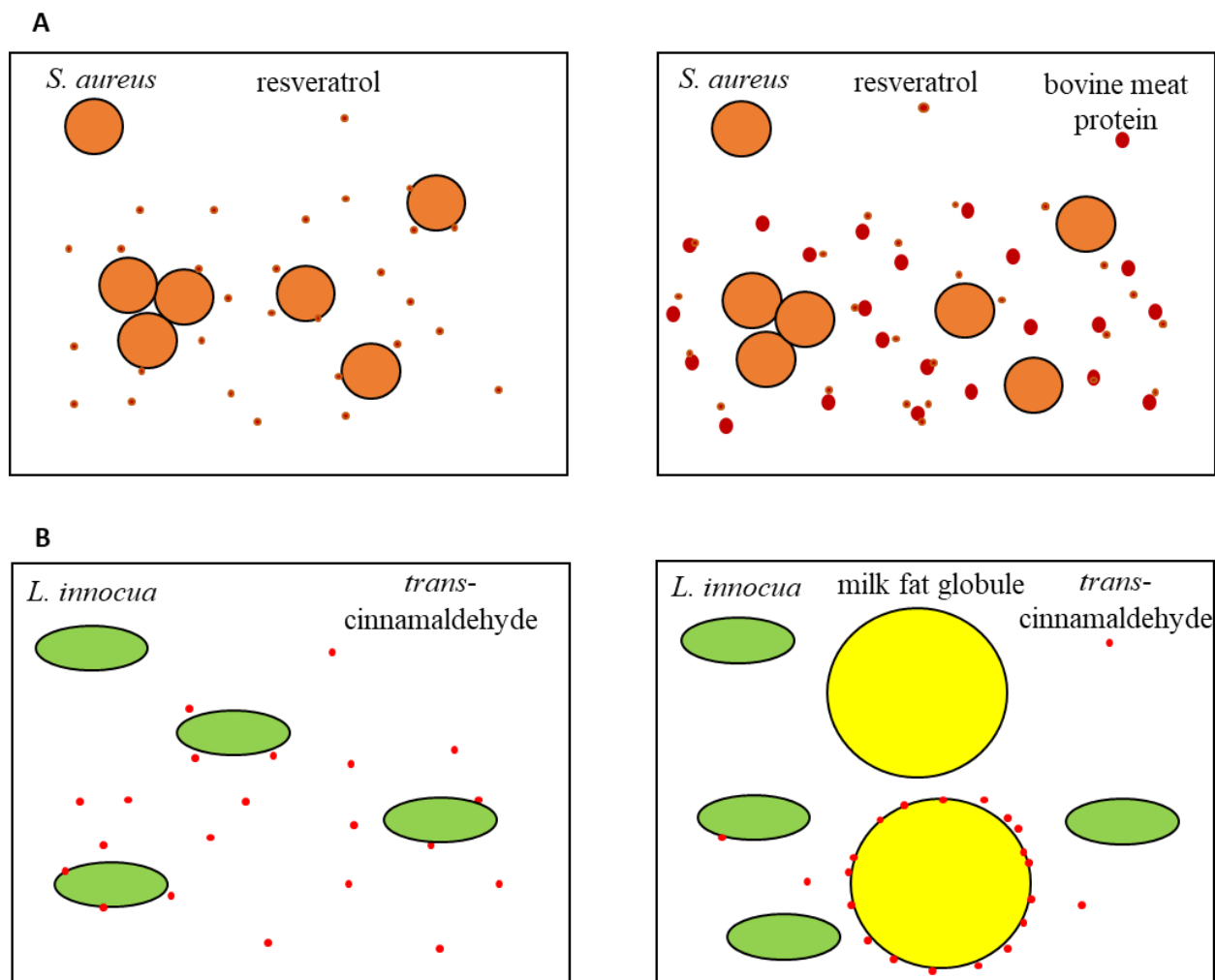
Figure 1. Scheme presenting interactions between resveratrol (as an example of polyphenol) and meat proteins ( A ) or between trans -cinnamaldehyde and milk fat globules ( B ) at the expense of interactions with S. aureus ( A ) or L. innocua ( B ) cells, respectively.
