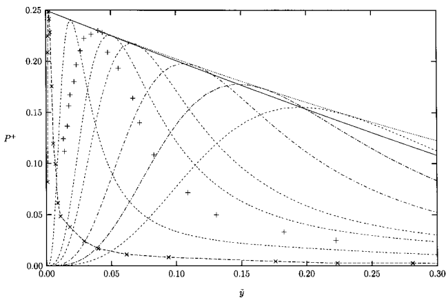
FIG. 4. Turbulent kinetic energy production in channel flow. Present study: ---, R^+ = 72 ; —, 90; - - -, 120; - · - ·, 180; - - - - -, 235; - - - - - · - - - - -, 590. Experimental data: (+), LDV measurements of Günter et al. (Ref. 10) at R^+ = 297 . (-×-×-) Comte-Bellot (Ref. 11), R^+ = 4800 . ···, P_p^+ [Eq. (3)], —, P_p^+ [Eq. (9)]. [The data from Comte-Bellot were obtained by differentiating the mean velocity profile and using Eq. (2).]
