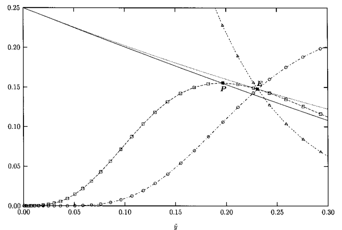
FIG. 2. Shear stresses and turbulent kinetic energy production from present DNS at R^+ = 72 . -Δ-Δ-, (S^+)^2 ; -○-○-, (\overline{uv}^+)^2 ; -□-□-, P^+ ; ···, P_E^+ [Eq. (3)]; —, P_P^+ [Eq. (9)].
