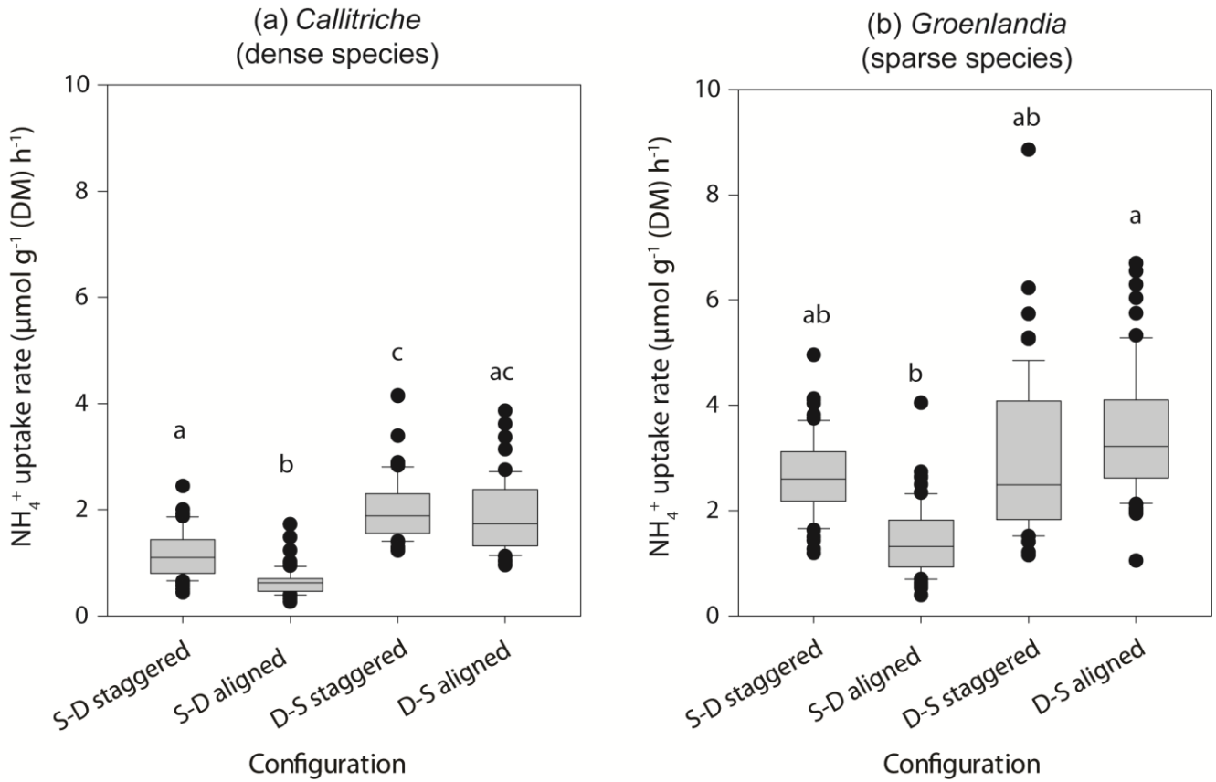
Figure 4 Boxplots of the distribution of \text{NH}_4^+ uptake rates ( \mu\text{mol g}^{-1} \text{ (DM) h}^{-1} ) within patches of the dense Callitriche (a) and the sparse Groenlandia (b) in each spatial configuration (S indicating sparse vegetation, D indicating dense vegetation, see Figure 2). Letters denote significant differences (Tukey's HSD, p < 0.05 ).
