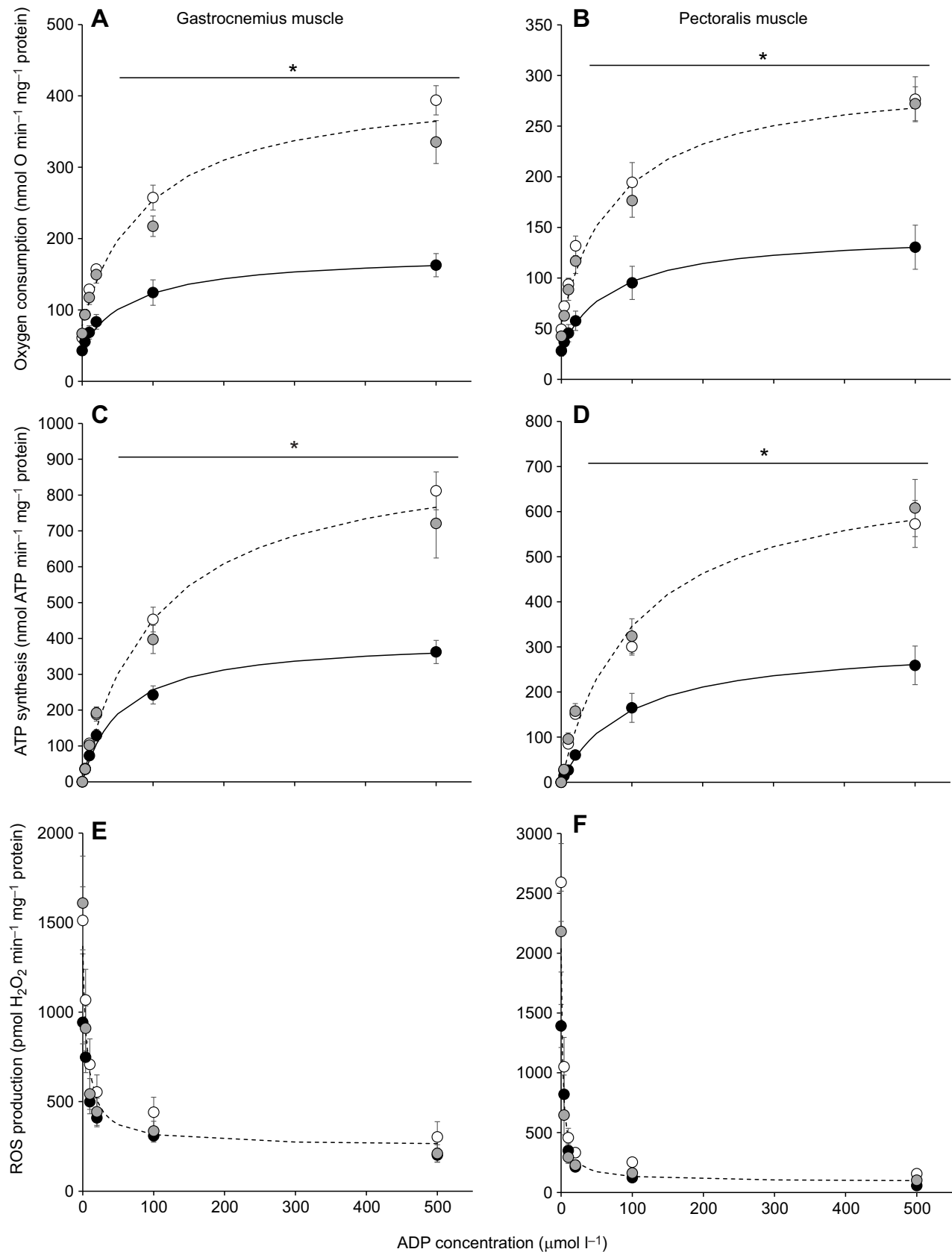
Fig. 1. Effect of fasting and refeeding on kinetic responses of oxygen consumption, ATP synthesis and H_2O_2 release to added ADP. Oxygen consumption (A,B), ATP synthesis (C,D) and H_2O_2 release (E,F) rates were determined at 40^\circ\text{C} in mitochondria respiring on pyruvate/malate/succinate and isolated from gastrocnemius (A,C,E) or pectoralis muscles (B,D,F) of fed (open circles), fasted (black circles) or re-fed (grey circles) ducklings. Values are means \pm s.e.m. for 6 animals. *Overall kinetic response to added ADP in fasted ducklings is significantly different from that of fed and re-fed ducklings ( P < 0.05 ).
