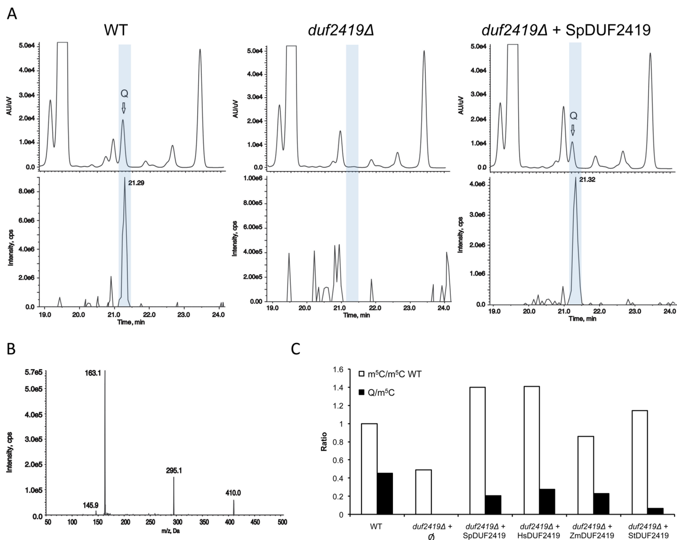
Figure 4. Results of LC–MS/MS analysis of S. pombe tRNA extracted from different strains. (A) Quantitation of queuosine (Q) content for different strains used in purified tRNA Asp GUC extracted from WT (left panel), duf2419Δ (middle panel), and duf2419Δ complemented with S. pombe DUF2419 (right panel, duf2419Δ + SpDUF2419). UV traces (top) at 254 nm and the extraction ion chromatograms (bottom) expected for Q ( [M + H]^+ m/z 410) are shown. (B) MS/MS fragmentation profile of m/z 410 confirming the identification of the nucleoside Q in the WT strain. The blue area highlights the elution time for queuosine. (C) Complementation of the Q - phenotype analyzed by LC–MS/MS. The ratios of Q/m 5 C in tRNA Asp GUC purified from the S. pombe WT strain and the duf2419Δ strain complemented with an empty vector ( duf2419Δ + ∅), S. pombe DUF2419 ( duf2419Δ + SpDUF2419), human DUF2419 ( duf2419Δ + HsDUF2419), maize DUF2419 ( duf2419Δ + ZmDUF2419), or S. thermophilus DUF2419 ( duf2419Δ + StDUF2419) are shown by the filled bars. To control for the amount of tRNA, the m 5 C content in the complemented strains was compared to the m 5 C content in the WT control (white bars). The results of a typical experiment are presented.
