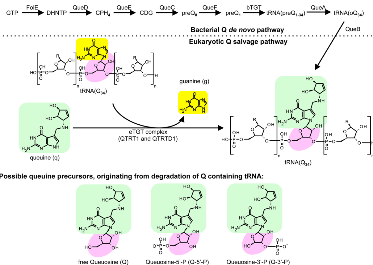
Figure 1. Queuosine structure and salvage pathway. Queuosine (Q) is synthesized de novo in bacteria. In eukaryotes, the last step of Q salvage occurs with the eukaryotic tRNA-guanine transglycosylase complex (eTGT) composed of QTRT1 and QTRTD1, responsible for the exchange of guanine (g) from a tRNA containing guanosine at position 34 (tRNA(G 34 )) with queuosine (q) to obtain a queuosine containing tRNA (tRNA(Q 34 )). Free queuosine (Q), queuosine-5'-phosphate (Q-5'-P), and queuosine-3'-phosphate (Q-3'-P) have been identified as possible precursors for Q salvage but the q conversion steps are unknown. Other abbreviations are GTP: guanosine-5'-triphosphate; DHNTP: 7,8-dihydroneopterin triphosphate; CPH 4 : 6-carboxy-5,6,7,8-tetrahydropterin; CDG: 7-carboxy-7-deazaguanine; preQ 0 : 7-cyano-7-deazaguanine; preQ 1 : 7-aminomethyl-7-deaza-guanine; tRNA(preQ 1-34 ): preQ 1 at the position 34 of tRNA; tRNA(oQ 34 ): epoxyqueuosine at the position 34 of tRNA; FolE: GTP cyclohydrolase-1; QueD: 6-carboxytetrahydropterin synthase; QueE: 7-carboxy-7-deazaguanine synthase; QueC: 7-cyano-7-deazaguanine synthase; QueF: 7-cyano-7-deazaguanine reductase; bTGT: bacterial type tRNA transglycosylase; QueA: tRNA (preQ 1-34 ) S-adenosylmethionine ribosyltransferase-isomerase; QueG: tRNA epoxyqueuosine (34) reductase.
