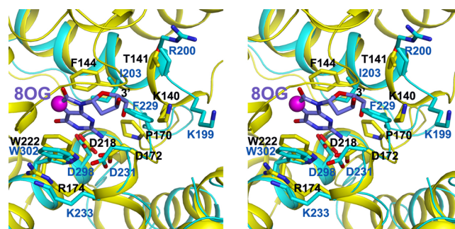
Figure 7. Homology model for the structure of the active-site in the DUF2419 protein from Sphaerobacter thermophilus (StDUF2419). The stereo ribbon diagram shows superposition of the homology model generated by PHYRE2 for StDUF2419 (the product of the Sthe_2331 gene, shown in cyan) with the template structure used to generate this model, 8-oxoguanine (8OG) DNA glycosylase from Pyrobaculum aerophilum (PDB 1XQO, shown in yellow). The 8OG molecule and the residues that interact with it in this structure are shown in ball-and-stick representation, along with the equivalent residues in the homology model of StDUF2419. Carbon atoms from the proteins are shown in the same color as the protein backbones, while carbon atoms from 8OG are shown in purple. Oxygen and nitrogen atoms are shown in red and blue, respectively. The 3' hydroxyl group of 8OG is labeled, while the magenta sphere indicates the location of the N7 atom of 8OG, which corresponds to the site of modification in queuosine.
