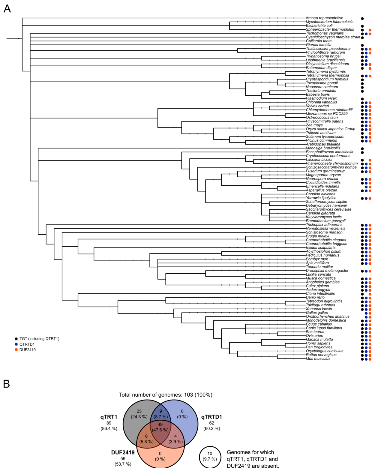
Figure 2. Taxonomic distribution of Q salvage genes. (A) Representative presence/absence pattern of TGT (including QTRT1, as they are in the same orthologous group in orthoMCL), QTRTD1, and DUF2419. Redundancy in clade has been limited. (B) Diagram presenting the full results of the distribution analysis from the data obtained at orthoMCL.org, enriched with NCBI Blast search for organism in which Q has been demonstrated present. Note that these representations are not informative of the number of gene occurrences per genome.
