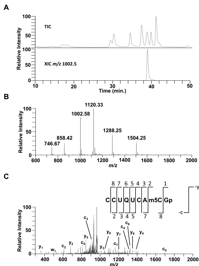
Figure 5. Schizosaccharomyces pombe tRNA Asp contains queuosine at position 34. (A) LC-MS/MS was performed on T1 digested tRNA producing a total ion chromatogram (TIC). (B) A digestion product ( m/z 1002.6) was found eluting at 39.0 min, as shown by the extracted ion chromatogram (XIC). The MS spectra at this time point depicts a signal from three oligonucleotides, CCU[Q]UCA[m 5 C]Gp ( m/z 1504.25 -2 and 1002.58 -3 ), AAUCCCg p ( m/z 1120.33 -2 and 746.67 -3 ), and UACACAAG>p ( m/z 1288.25 -2 and 858.42 -3 ). (C) Collision induced dissociation of m/z 1002.58 produces the nearly all expected -c and -y ions for the sequence CCU[Q]UCA[m 5 C]Gp.
