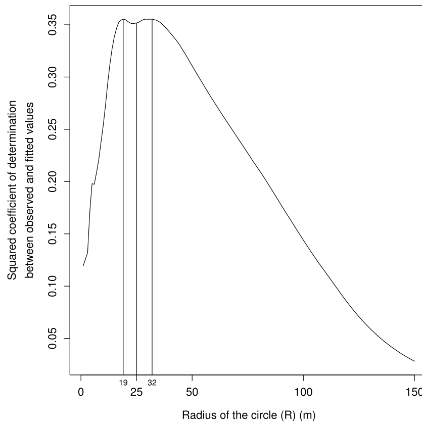
Figure 4 Squared coefficients of determination between the observed and the fitted values for models built with values of unobstructed areas calculated for circles of radii (R in Fig. 1, in m) ranging from 1 to 150 m and plotted on x axis. The biologically relevant distance ranges between 19 and 32 m, in line with our field observations of cat hunting bouts.
