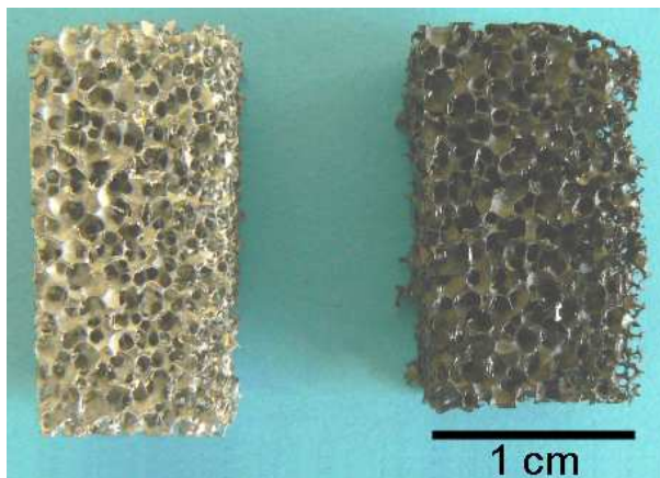
Figure 3: Stainless steel foam before (left) and after carbon coating (right) by the polymerisation method.
