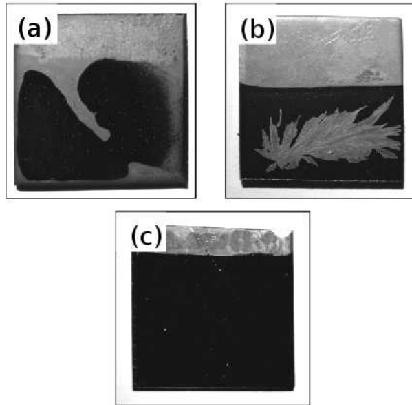
Figure 2: Pictures of samples without (a, b) and with stainless steel pretreatment (c).
