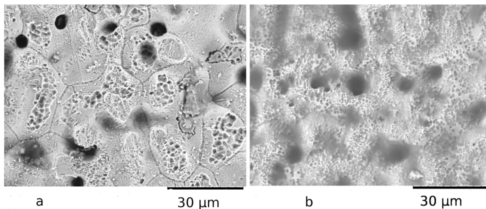
Figure 5: SEM pictures of stainless steel foam before (a) and after (b) carbon coating (suspension method with 2% dextrine).
