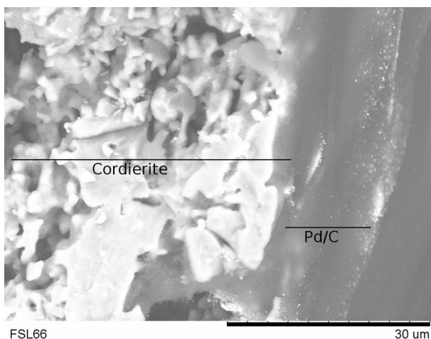
Figure 6: Cross section SEM picture of cordierite monolith after Pd/C coating by suspension method.
