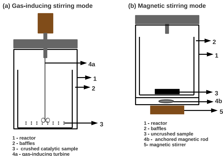
Figure 1: Nitrobenzene hydrogenation reactor with two stirring modes (a - gas-inducing stirring mode and b - magnetic stirring).
