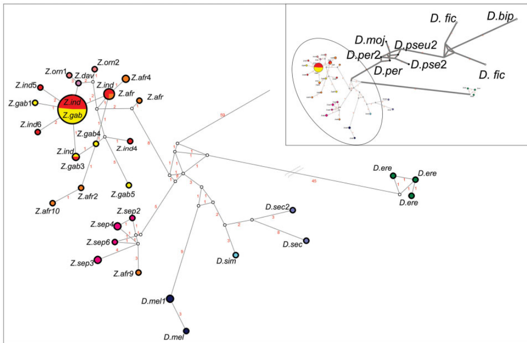
Fig. 5. —Phylogenetic network reconstruction for the non-LTR retrotransposon BS of Zaprionus and Drosophila species with emphasis on the relationships between the sequences of Zaprionus and the species of the melanogaster complex. The network was constructed with amino acid sequences of the reverse transcriptase gene using the median-joining algorithm implemented in Network 5.0.0.1 (Bandelt et al. 1999). The size of each circle denotes the number of sequences grouped together, and the branch lengths are proportional to the number of substitutions between two nodes. Small empty circles represent the ancestor vectors, black circles represent sequences that do not belong to the melanogaster group, and grey circles represent sequences that belong to the melanogaster group from the Oriental region. The sequences from the melanogaster subgroup are represented by cool colors (blue to green), and Zaprionus sequences are represented by warm colors (red to purple). Z. ind : Z. indianus , Z. gab : Z. gabonicus , Z. afr : Z. africanus , Z. sep : Z. sepsoides , Z. dav : Z. davidi , Z. om : Z. ornatus , D. mel : D. melanogaster , D. sim : D. simulans , D. sec : D. sechellia , D. ere : D. erecta , D. bip : D. bipunctinata , D. fic : D. ficusphila , D. per : D. persimilis , D. pse : D. pseudoobscura , and D. moj : D. mojavensis . This analysis used 227 codons and 67 sequences.
