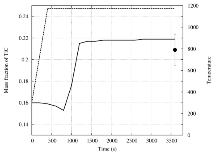
Fig. 11 Change in the calculated TiC mass fraction during heat treatment of a composite powder compact prior to the consolidation step (solid line). Temperature vs time is also reported (dashed line) as well as the experimental mass fraction determined after heat treatment and the consolidation step (filled circle).
