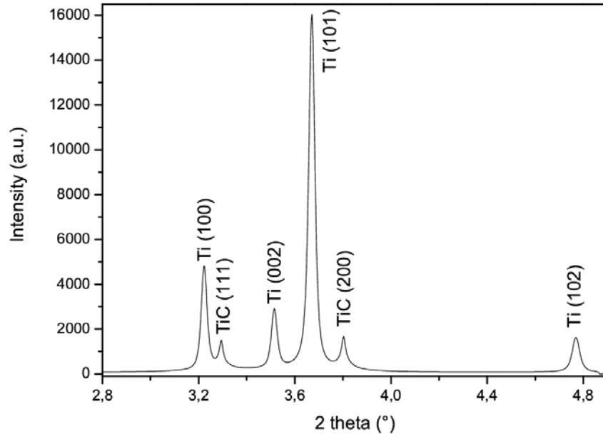
Fig. 1 Example of diffraction pattern collected from the sample at room temperature with peak identification
