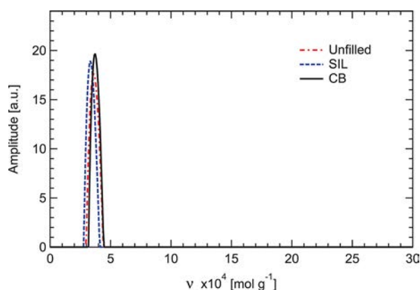
Figure 7. Distributions of cross-link density \nu in a pure, unfilled NR sample (1.0 phr S) and in SIL and CB filled materials (1.5 phr S), which have roughly the same average values \nu \approx 3.5 \times 10^{-4} \text{ mol}\cdot\text{g}^{-1} . No contribution from regions with cross-link densities up to 10 times the average value is observed.
