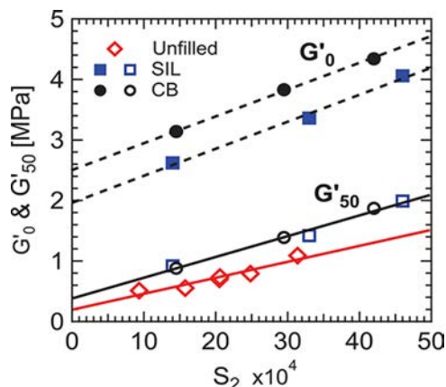
Figure 6. Storage shear moduli G'_0 (full symbols) and G'_{50} (empty symbols) for the 12 different studied samples, as a function of the slope S_2 of \langle P_2 \rangle measured by X-ray scattering: unfilled ( \diamond ), SIL ( \square ), and CB ( \circ ) samples.
