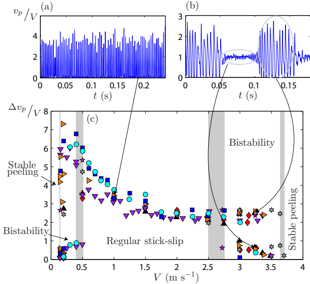
Figure 2: Portions of the measured time series v_p(t)/V for typical experiments at \theta = 90^\circ : (a) L = 45 cm, V = 1 \text{ m s}^{-1} , regular stick-slip; (b) L = 69 cm, V = 3.25 \text{ m s}^{-1} , bistable peeling. (c) Statistical average \Delta v_p/V of the amplitude of fracture velocity fluctuations \delta v_p(t)/V as a function of V for \theta = 90^\circ and various peeled tape lengths L ( \blacklozenge : L = 25 cm ; \blacktriangle : L = 34 cm; \blackstar : L = 45 cm; \blacktriangledown : L = 54 cm; \blacktriangleright : L = 69 cm; \blackstar : L = 81 cm; \blacksquare : L = 100 cm; \bullet : L = 134 cm). The standard deviation of \delta v_p(t)/V over all velocity fluctuations in one experiment is typically of the order of the symbol size.
