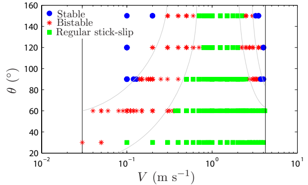
Figure 3: Diagram of the peeling regime in (V, \theta) -space. Each marker corresponds to one experiment. The vertical lines show the experimental limits of our setup. Continuous grey lines are guides for the eyes.
