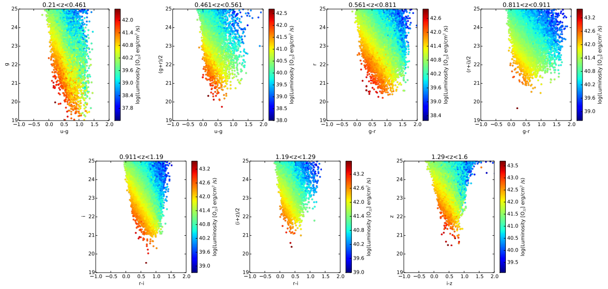
Fig. A.1. Predictions from the CMC for magnitude vs. color (in the CFHT system) and observed [OIII] luminosity for the CFHT magnitude redshift bins described in Table 5 and Fig. 12.
