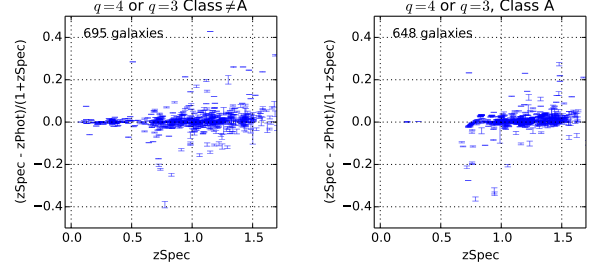
Fig. 5. Comparison between the spectroscopic redshift and photometric redshift.
