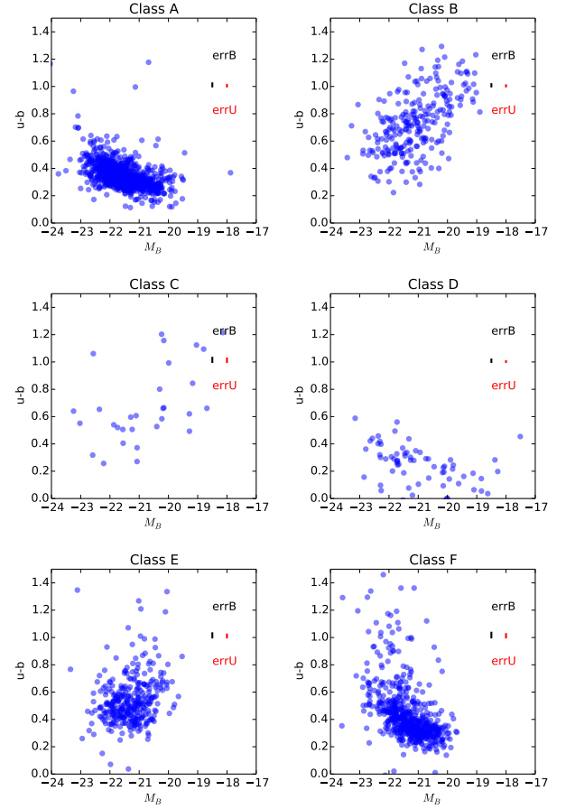
Fig. 2. Selection. u-b color vs. M_B absolute magnitude for each selection with M_B derived using the photometric redshift. The vertical bars show the mean 1\sigma error on the u and b bands for each selection. Class A objects are bright and blue.
