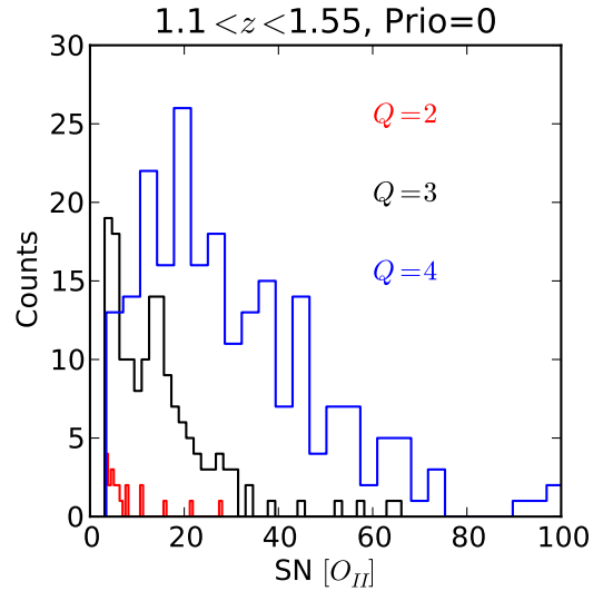
Fig. 6. SNR in the [OII] lines for different redshift quality flags. The galaxies with Q = 3 or 4 are used to determine the luminosity function.
