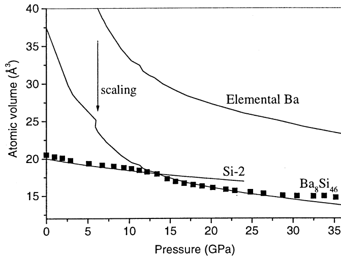
FIGURE 2 Comparison between the evolution of the atomic volume in \text{Ba}_8\text{Si}_{46} (squares), Si-2 and elemental Ba. This last one is also shown scaled by a factor 0.59 to match the atomic volume of \text{Ba}_8\text{Si}_{46} at the pressure instability (13 GPa).
