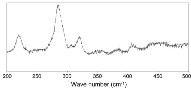
Fig. 3. Raman spectrum of Mo-S-I nanowires.
